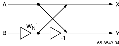
Figure 6. Signal Flow of Radix-2 Butterfly
