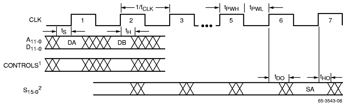
Figure 4. Timing Diagram
