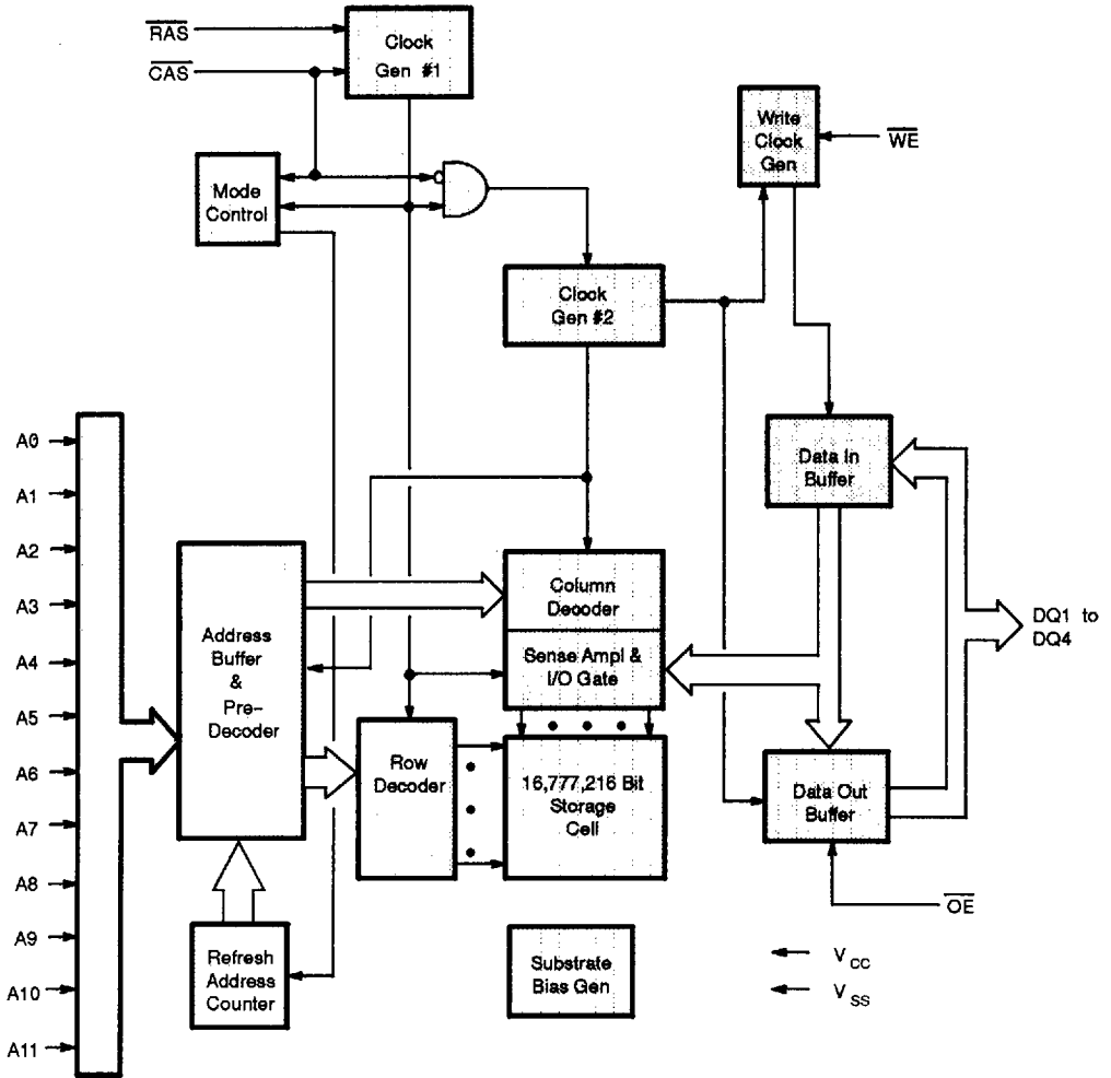
Fig. 1 - MB8116400A DYNAMIC RAM - BLOCK DIAGRAM
