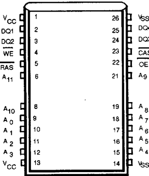
26/24-Pin SOJ : (TOP VIEW)
