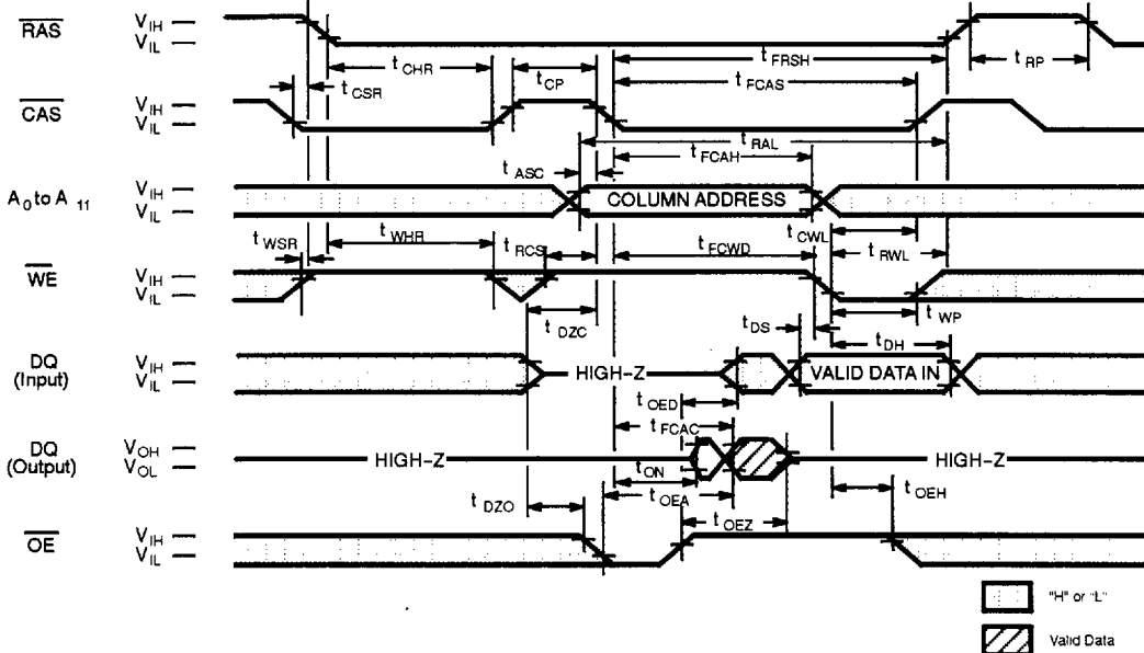
Fig. 16 - CAS-BEFORE-RAS REFRESH COUNTER TEST CYCLE
