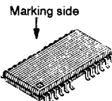
Plastic TSOP Packages (FPT-26P-M05) (Normal Bend) (Reverse Bend)
