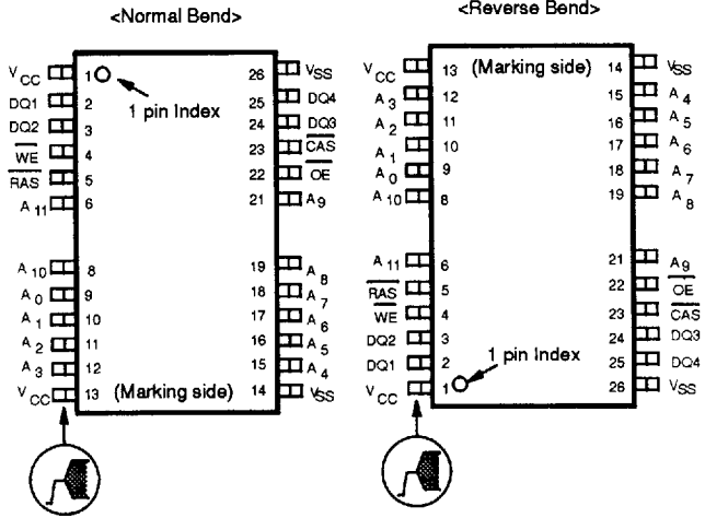
26/24-Pin FPT (TOP VIEW)
