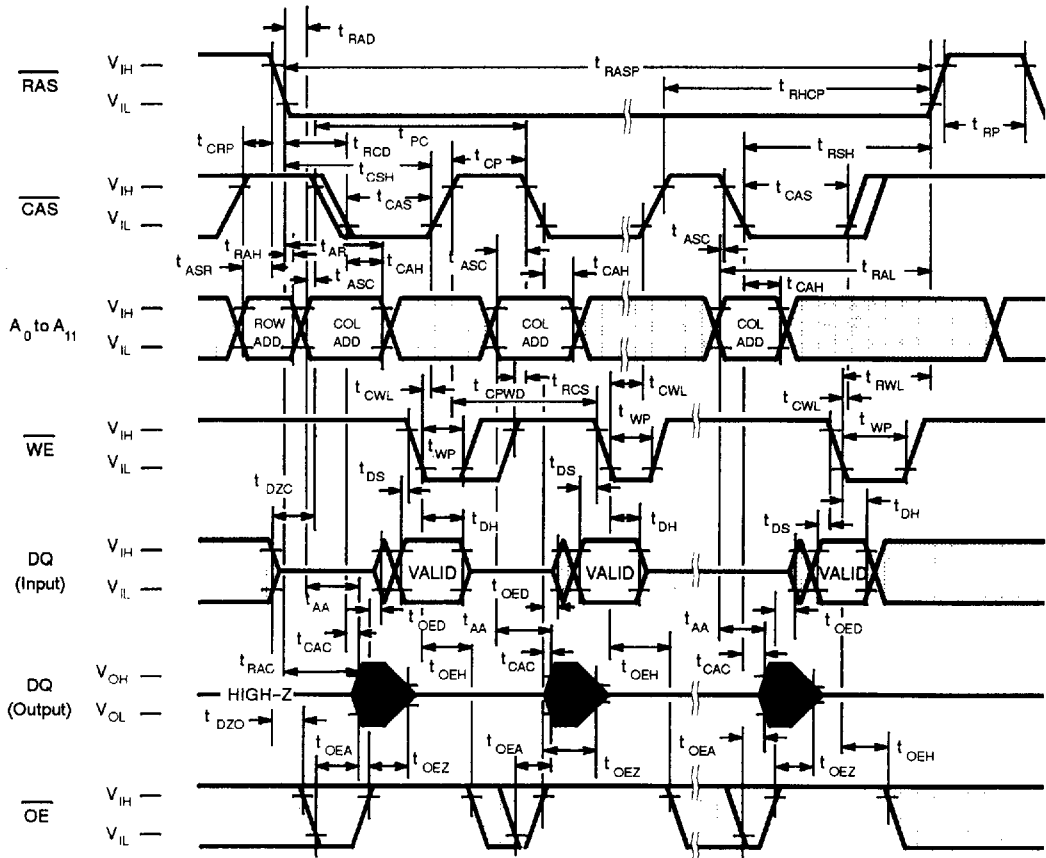
Fig. 10 — FAST PAGE MODE \overline{OE} WRITE CYCLE
