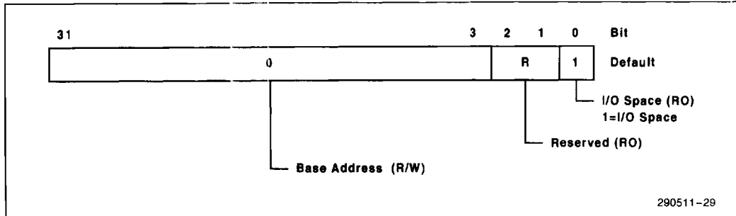
Figure 13. IDE Base Address Register 0
