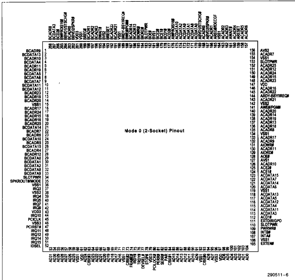
Figure 4. Mode 0 Pinout
