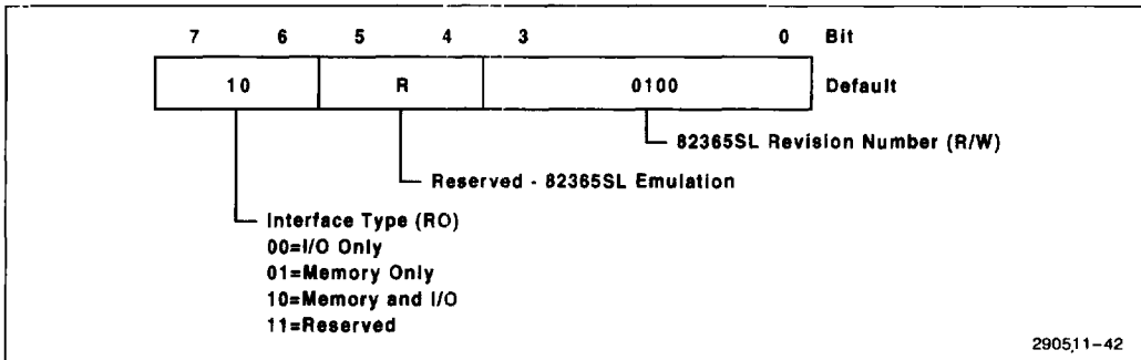
Figure 24. Identification Register
