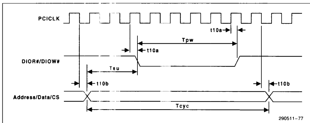
Figure 45. IDE Timing
