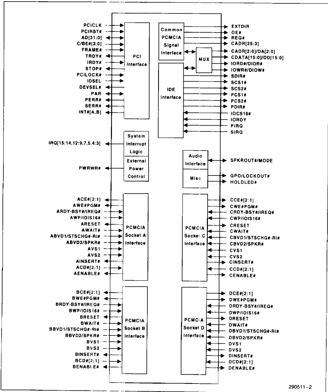
Mode 1 (Four Socket) Block Diagram
