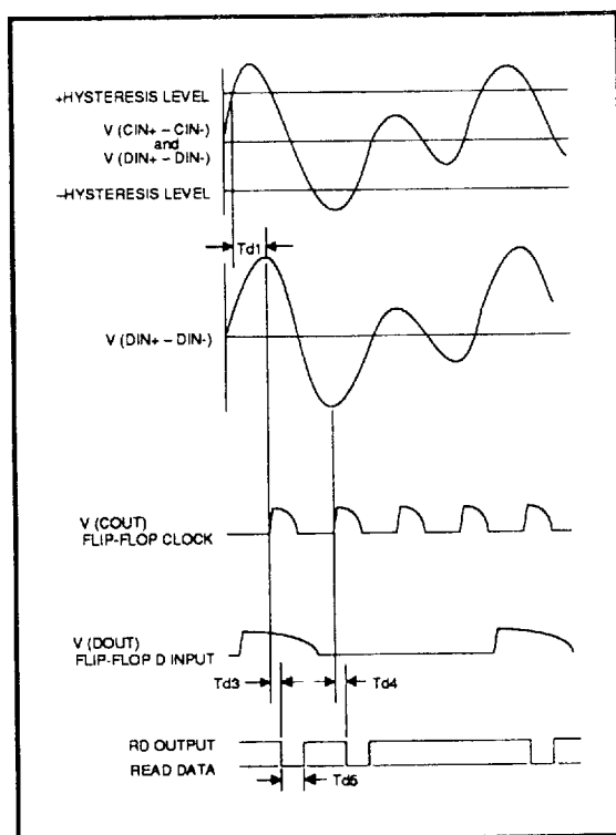
FIGURE 2: Timing Diagram
