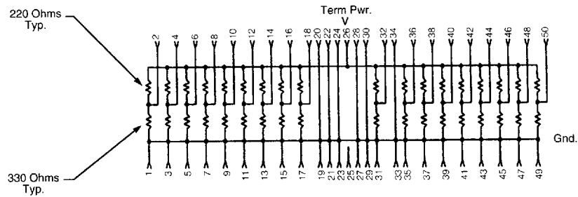
50-Position, Single-Ended Part No. 869036-1
