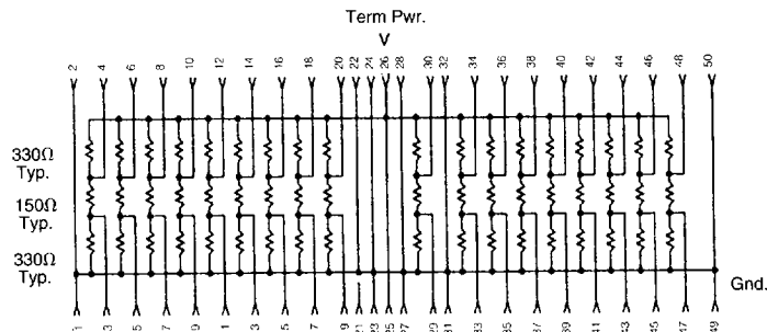
50-Position, Differential Part No. 869041-1
