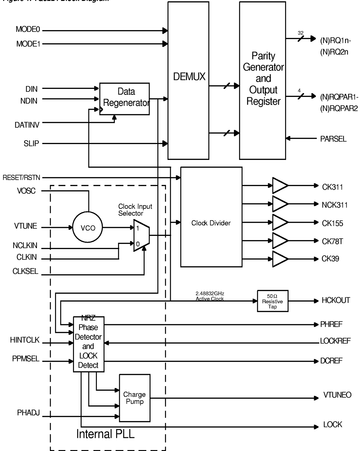
Figure 1. TQ8224 Block Diagram
