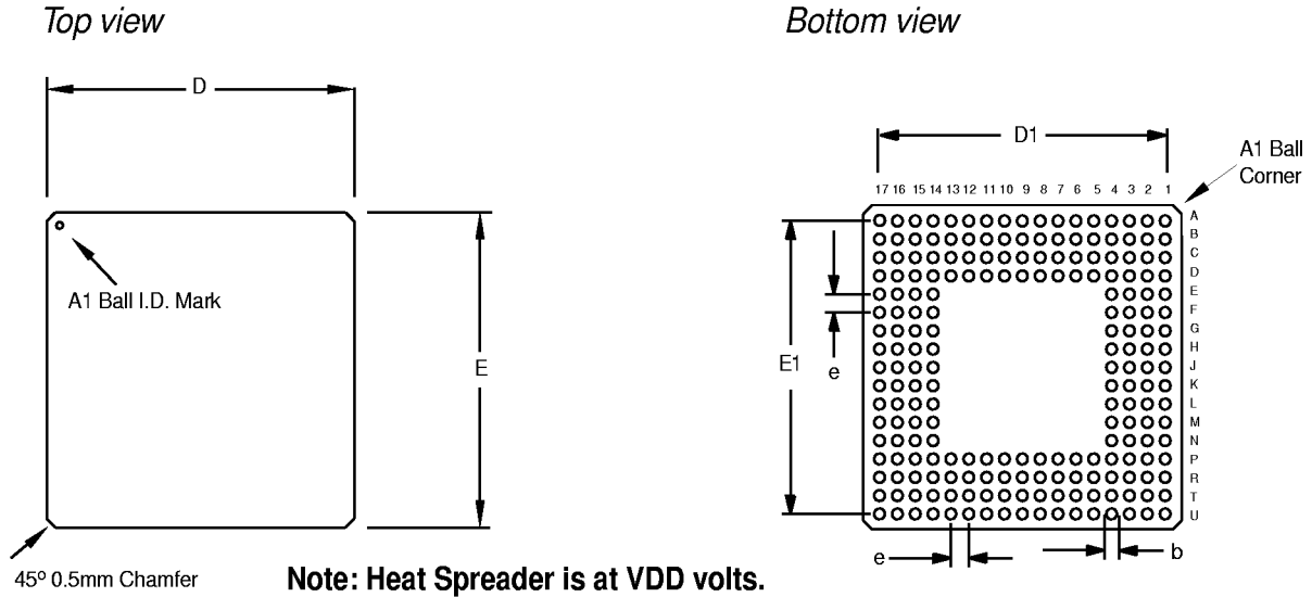
Figure 11. 208-pin BGA Mechanical Dimensions
