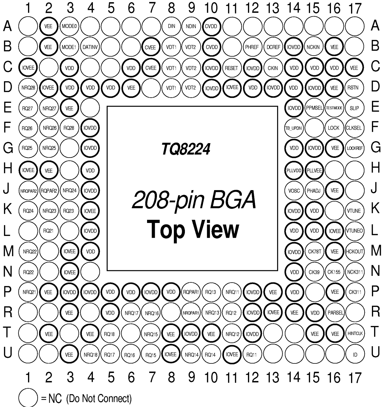
Figure 3. TQ8224 Pinout - Top View
