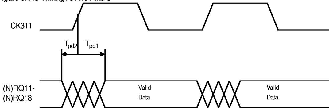
Figure 6. AC Timing: 311.04 Mb/s
