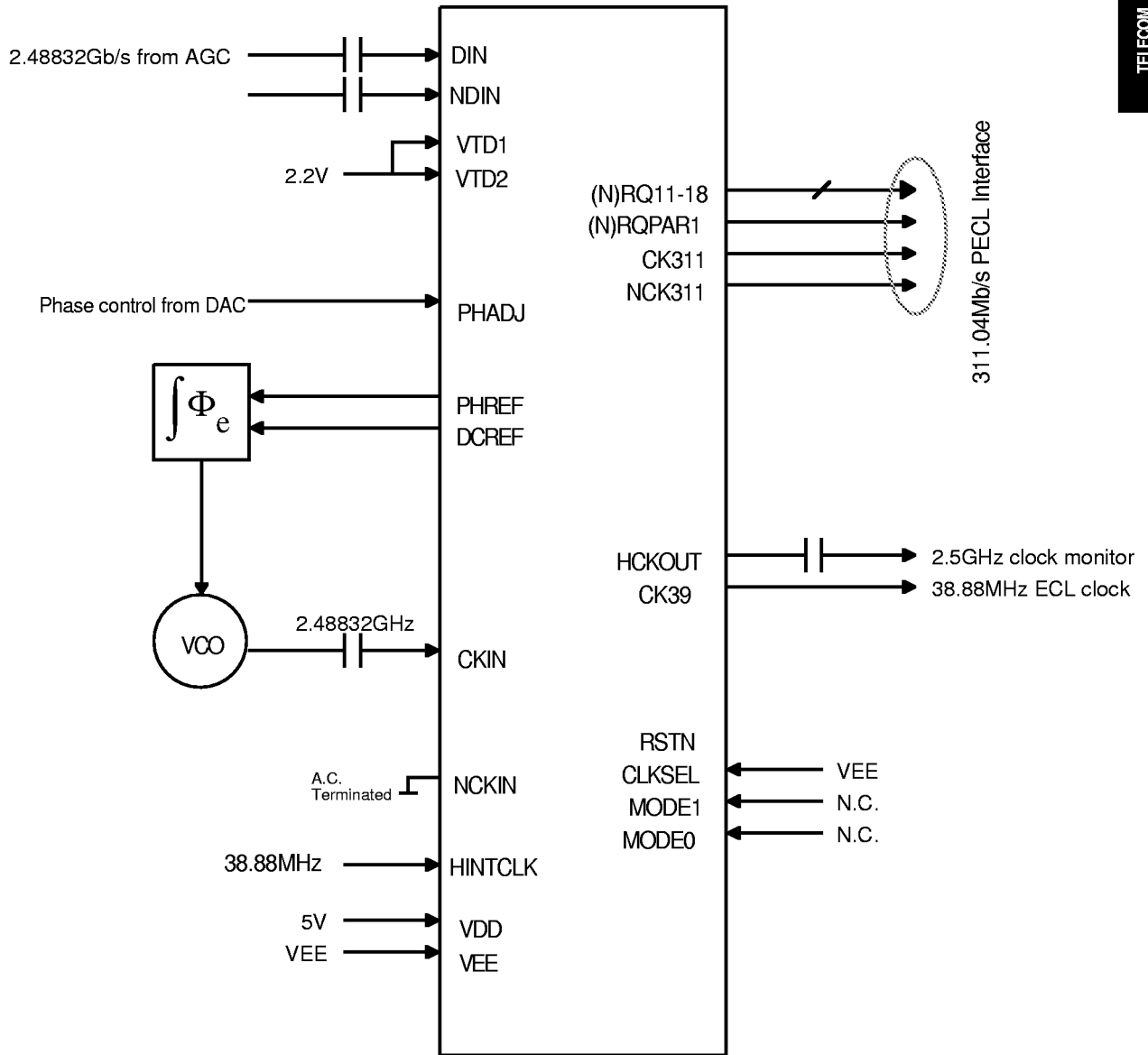
Figure 9. 1:8 Demultiplexing with External PLL and VCO
