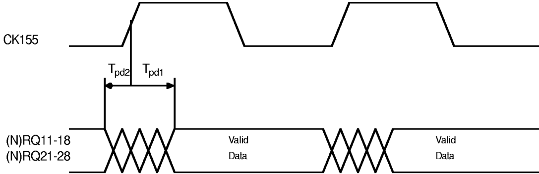
Figure 7. AC Timing: 155.52 Mb/s Interface
