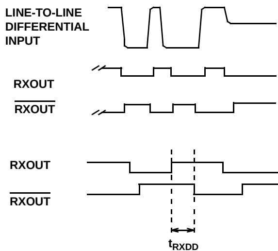
Figure 4. Typical Receiver Waveforms
