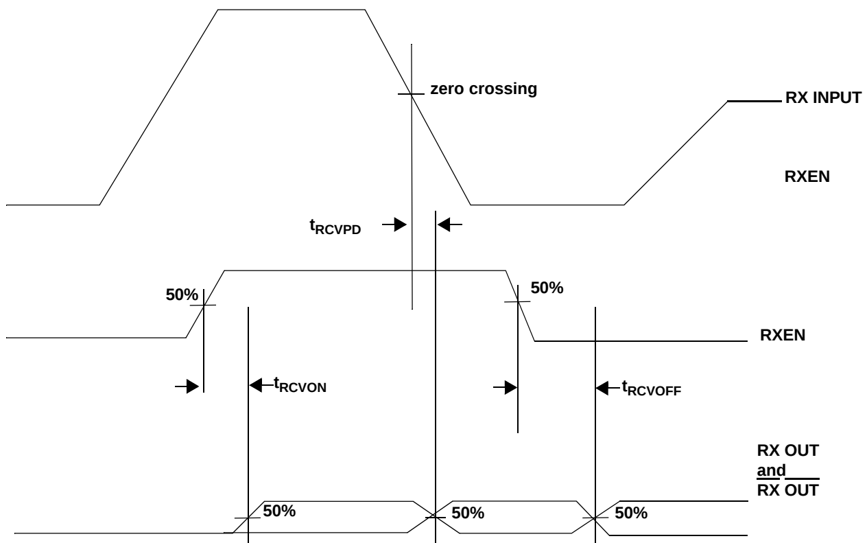
Figure 13. Receiver Timing
