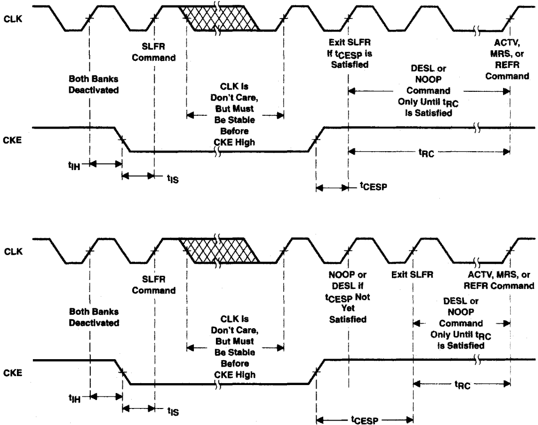
Figure 19. Self-Refresh Operation
