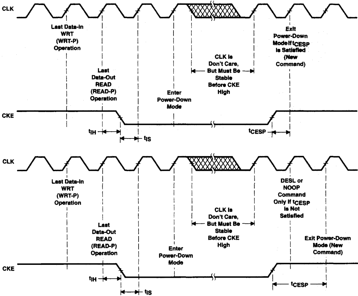
Figure 18. Power-Down Operation
