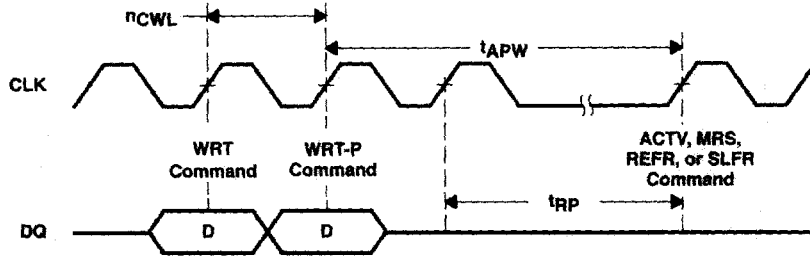
Figure 15. Write With Auto-Deactivate
