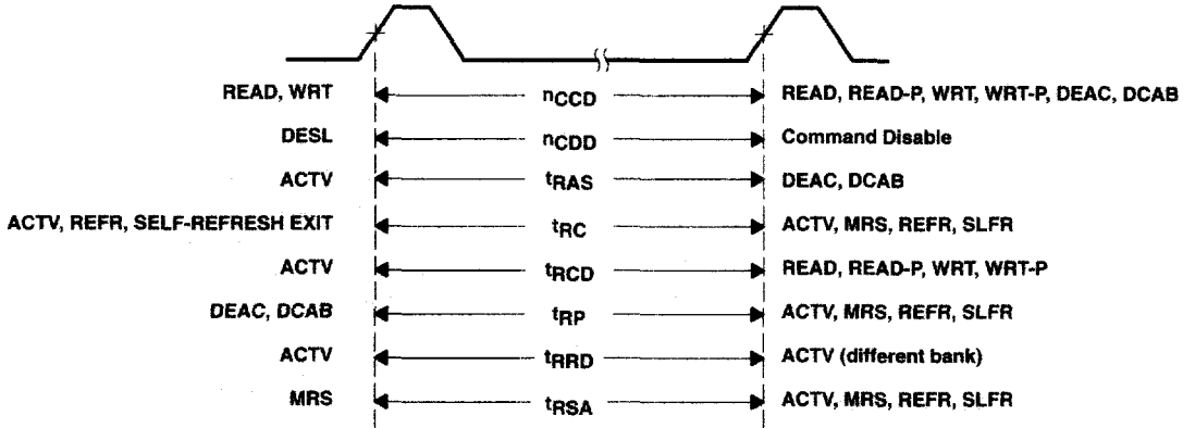
Figure 11. Command-to-Command Parameters
