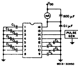
Fig. 17 - Dynamic power dissipation test circuit.
