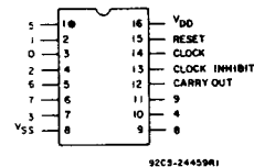
TOP VIEW CD4017B TERMINAL DIAGRAM
