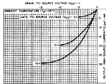
Fig. 7— Typical output high (source) current characteristics.
