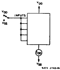
Fig. 14 - Quiescent device-current test circuit.
