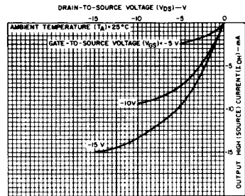
Fig. 8— Minimum output high (source) current characteristics.
