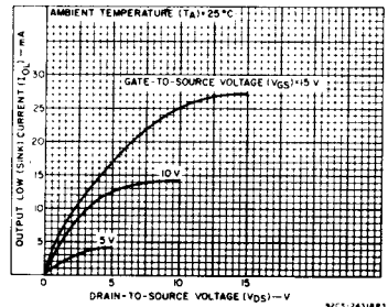
Fig. 5— Typical output low (sink) current characteristics.
