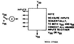
Fig. 15 - Input-leakage current.
