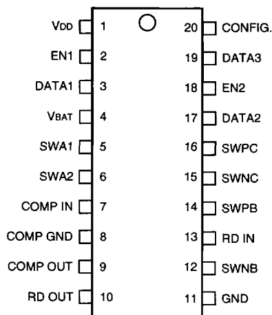
Figure 2. Pin Diagram
