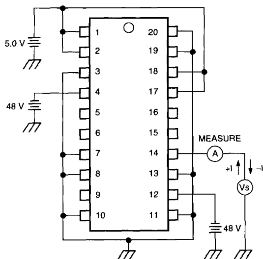
Figure 16. High-Voltage Leakage Current — Switch B
