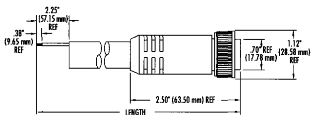
Straight Female Plug
