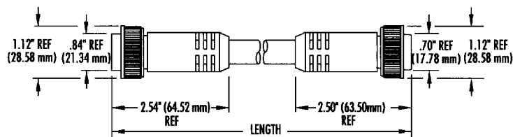
Male/Female Cable Assembly
