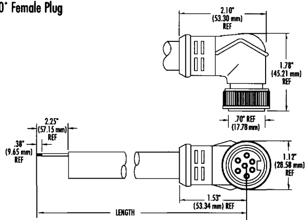
90° Female Plug
