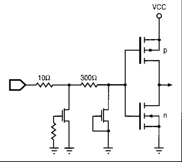
FIGURE 2. OUTPUT CIRCUIT
