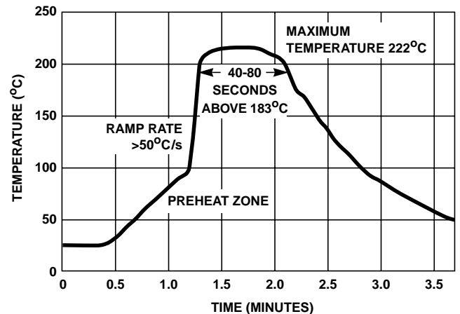
FIGURE 9. VAPOR PHASE SOLDER PROFILE
