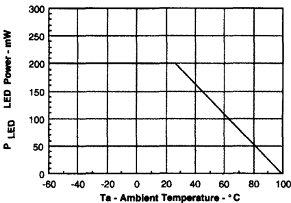
Figure 6. Maximum output power dissipation
