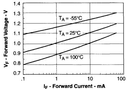
Figure 2. Forward voltage versus forward current
