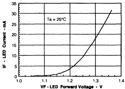
Figure 1. LED forward current vs. forward voltage
