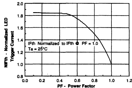
Figure 8. Normalized LED trigger current
