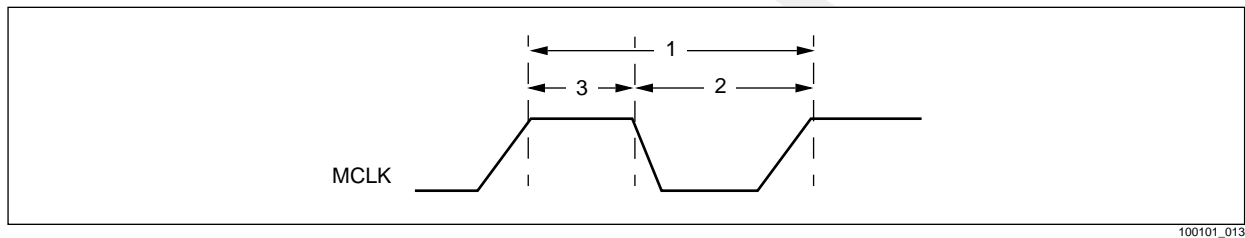
Figure 5-1. MCLK Timing Requirements
