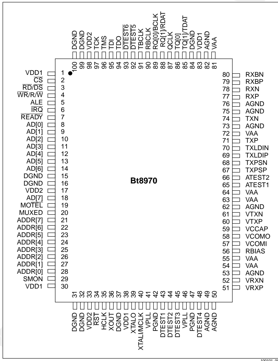
Figure 1-3. Pin Diagram
