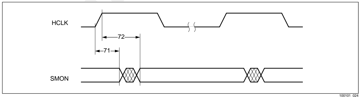
Figure 5-12. SMON Timing
