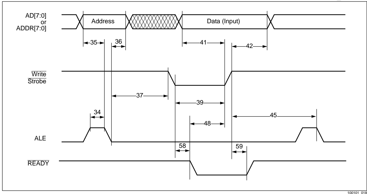
Figure 5-6. MCI Write Timing, Intel Mode (MOTEL = 0)
