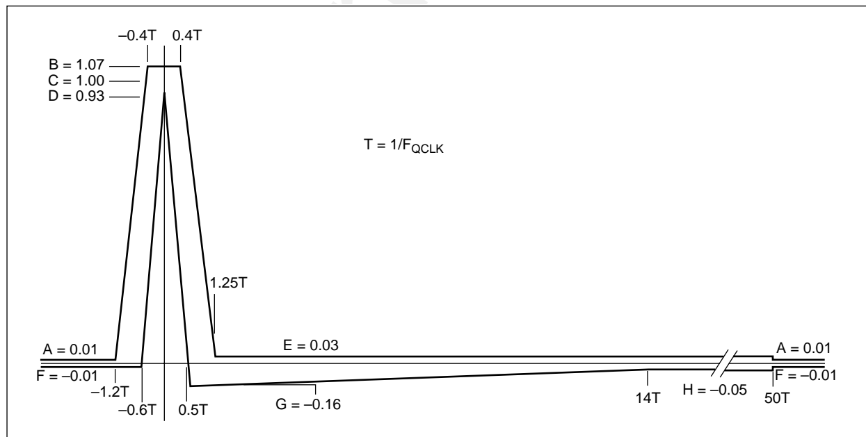
Figure 5-13. Transmitted Pulse Template
