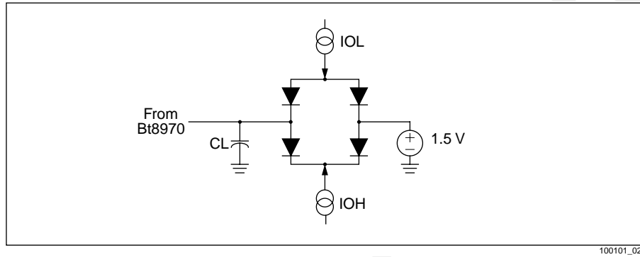
Figure 5-15. Standard Output Load (Totem Pole and Three-State Outputs)
