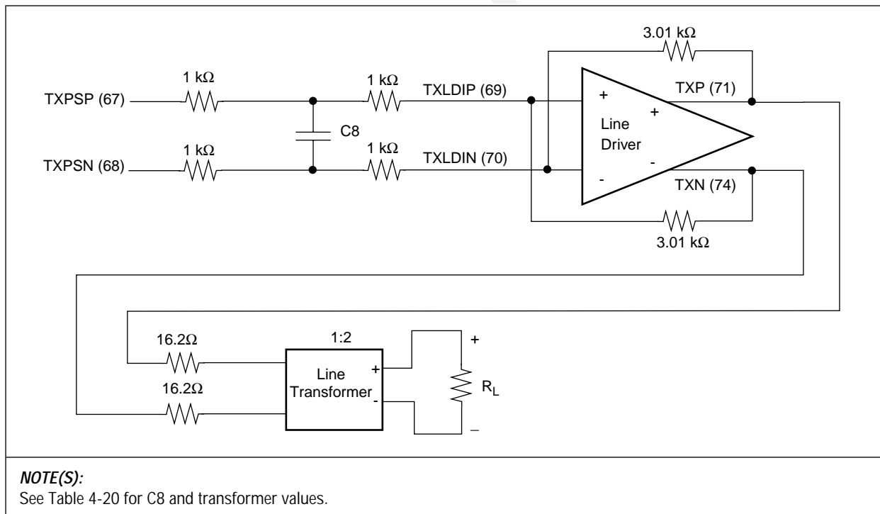
Figure 5-14. Transmitter Test Circuit
