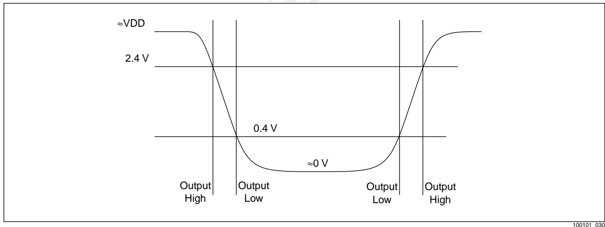
Figure 5-18. Output Waveforms for Timing Tests
