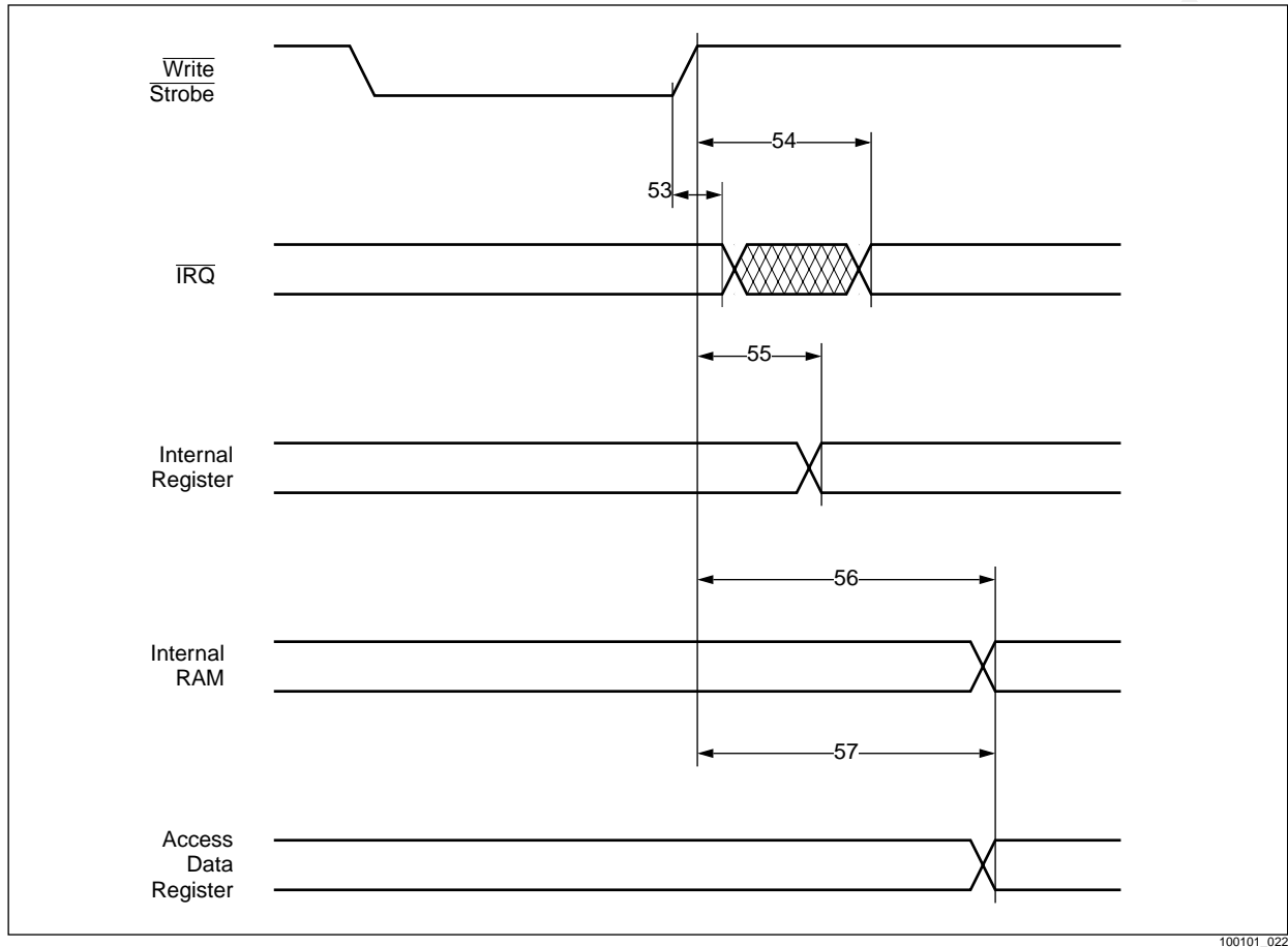
Figure 5-10. Internal Write Timing
