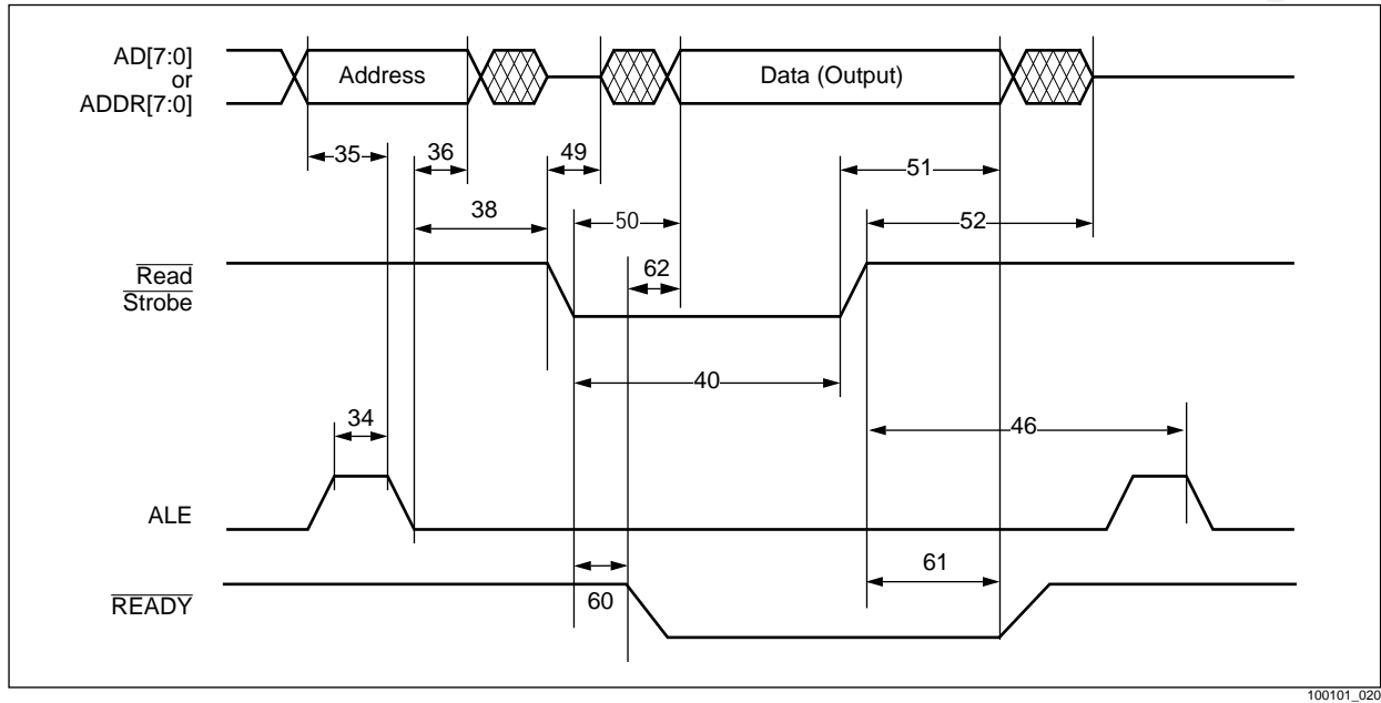
Figure 5-8. MCI Read Timing, Intel Mode (MOTEL = 0)
