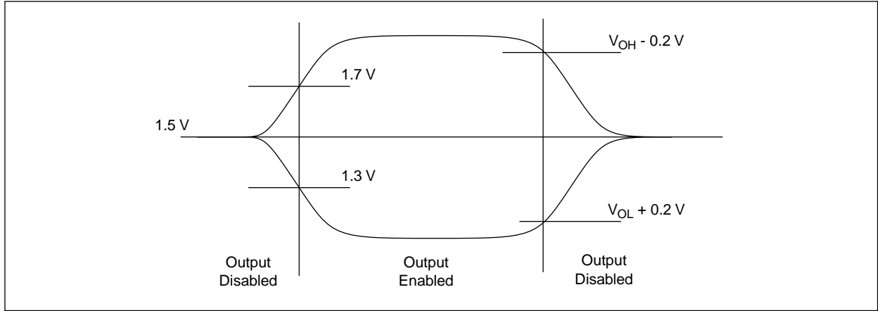
Figure 5-19. Output Waveforms for Three-state Enable and Disable Tests
