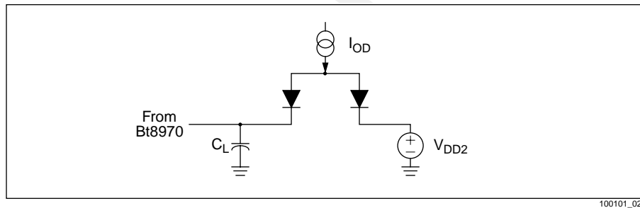
Figure 5-16. Open-Drain Output Load ( \overline{IRQ} )
