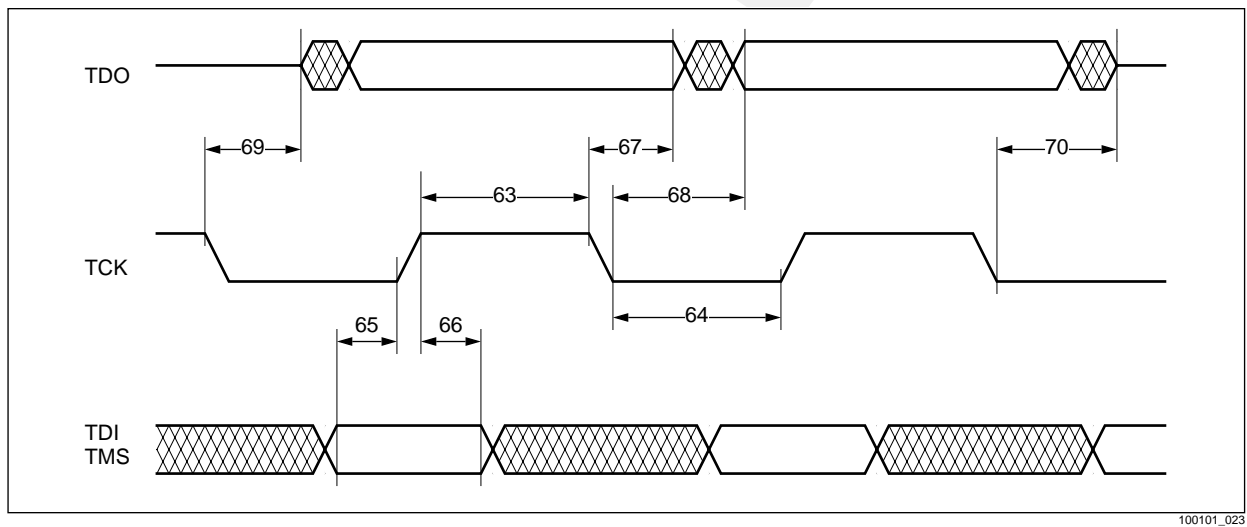
Figure 5-11. JTAG Interface Timing
