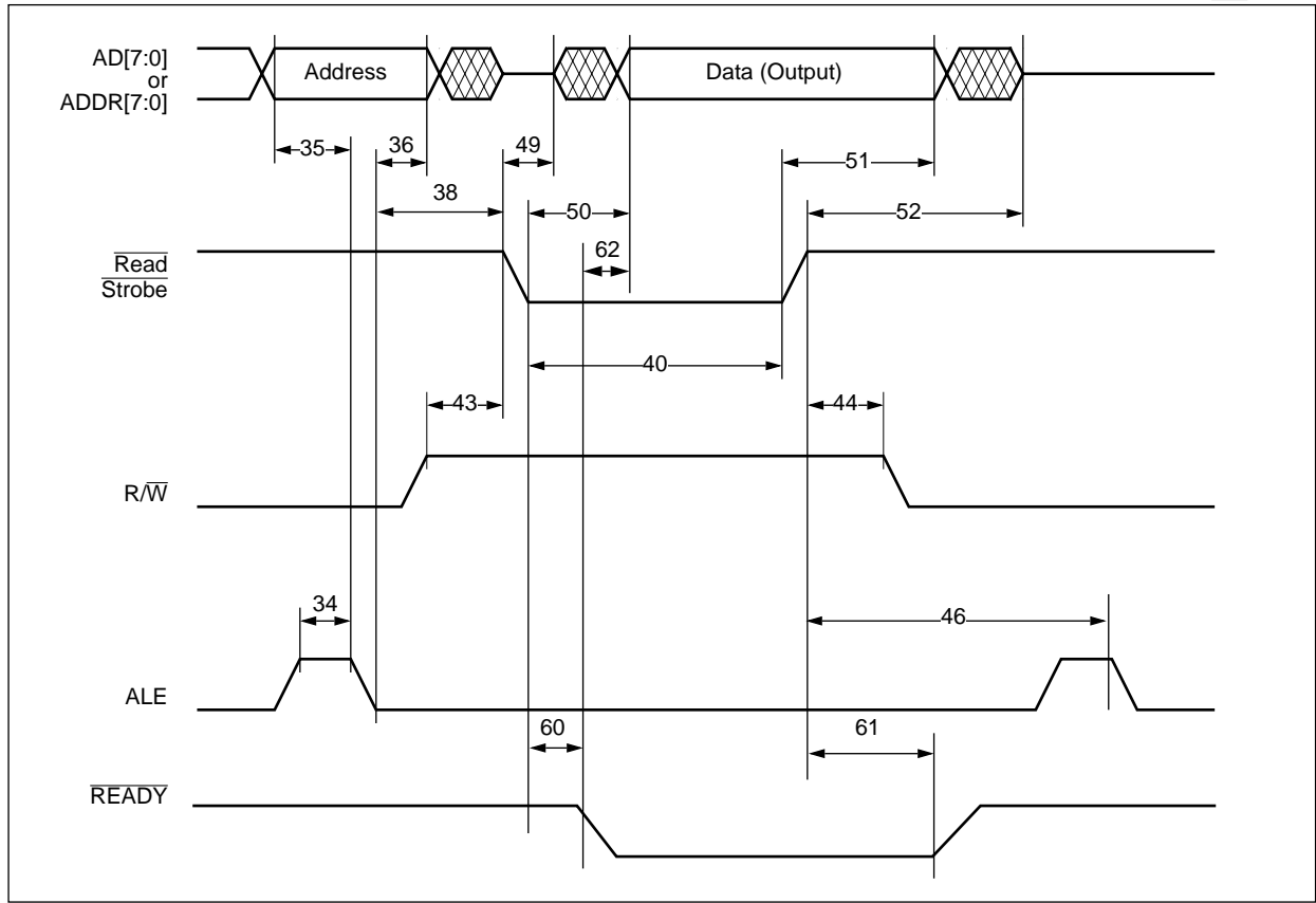
Figure 5-9. MCI Read Timing, Motorola Mode (MOTEL = 1)
