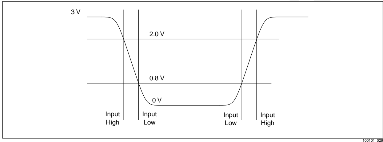
Figure 5-17. Input Waveforms for Timing Tests
