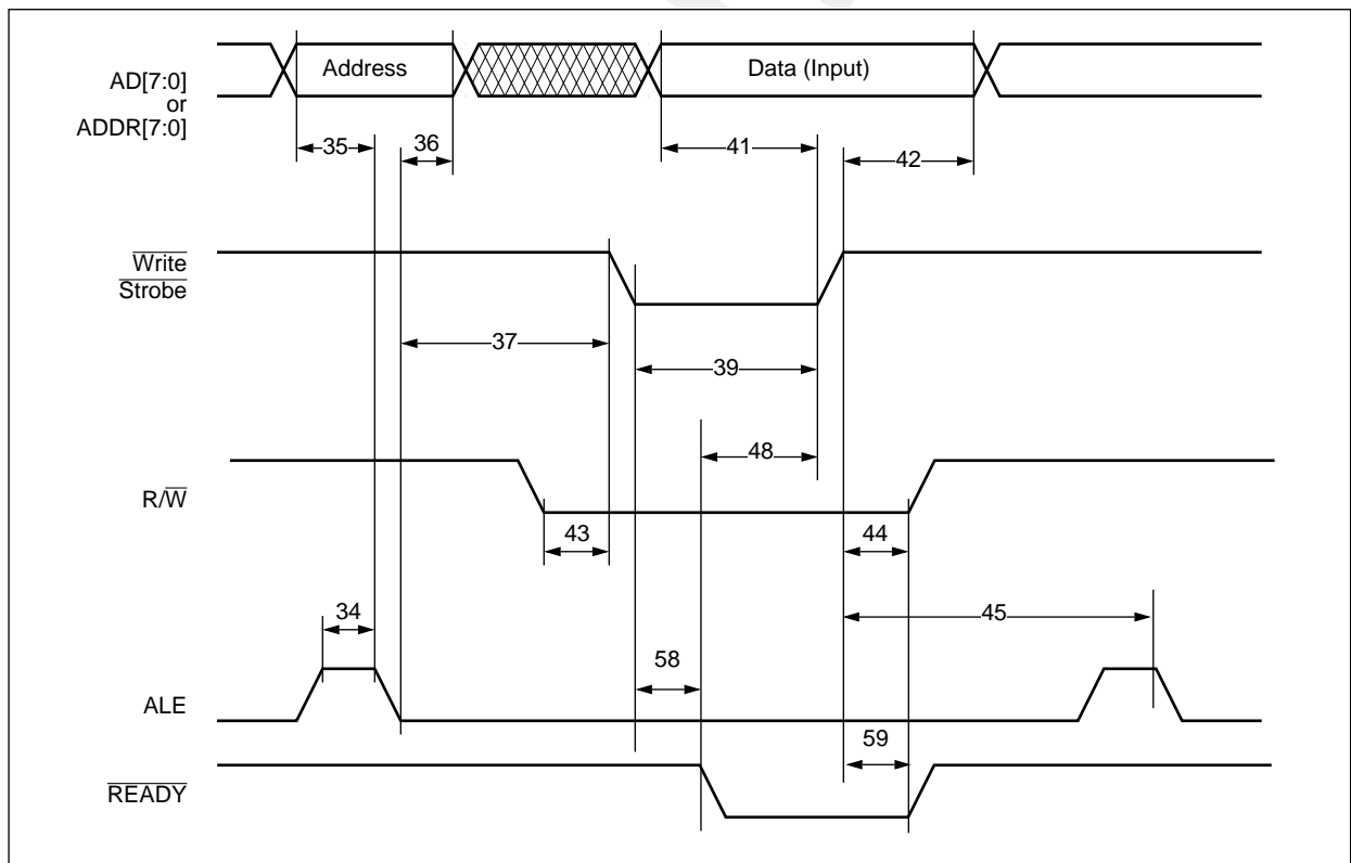
Figure 5-7. MCI Write Timing, Motorola Mode (MOTEL = 1)
