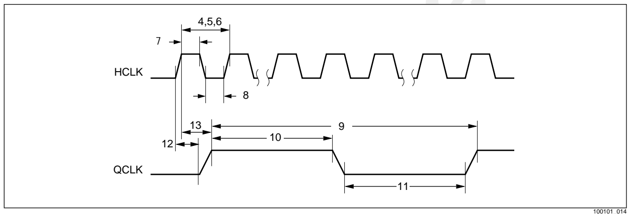
Figure 5-2. Clock Control Timing
