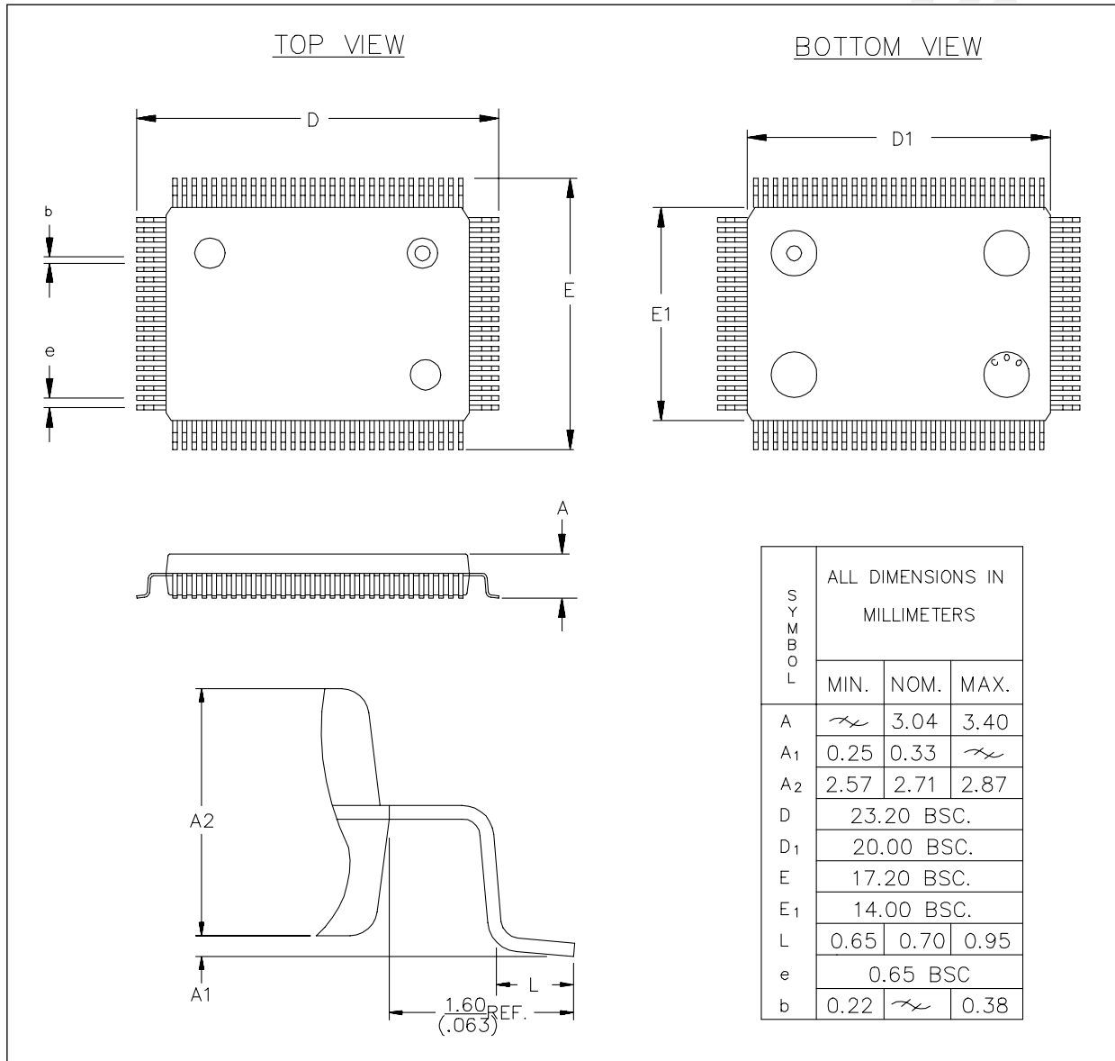
Figure 5-20. 100-Pin Plastic Quad Flat Pack (PQFP)
