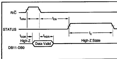
FIGURE 2. R/C Pulse High — Outputs Enabled Only While R/C is High.
