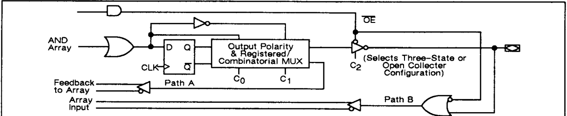
Figure 2. General Output Macrocell Diagram. Applies to macrocells with 64mA outputs. 48mA output macrocells are three-state regardless of the state of C_2 .
