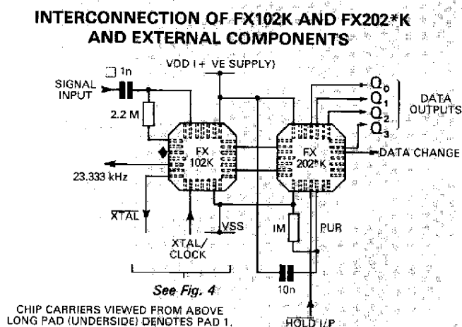
Fig. 3 Chip Carrier
