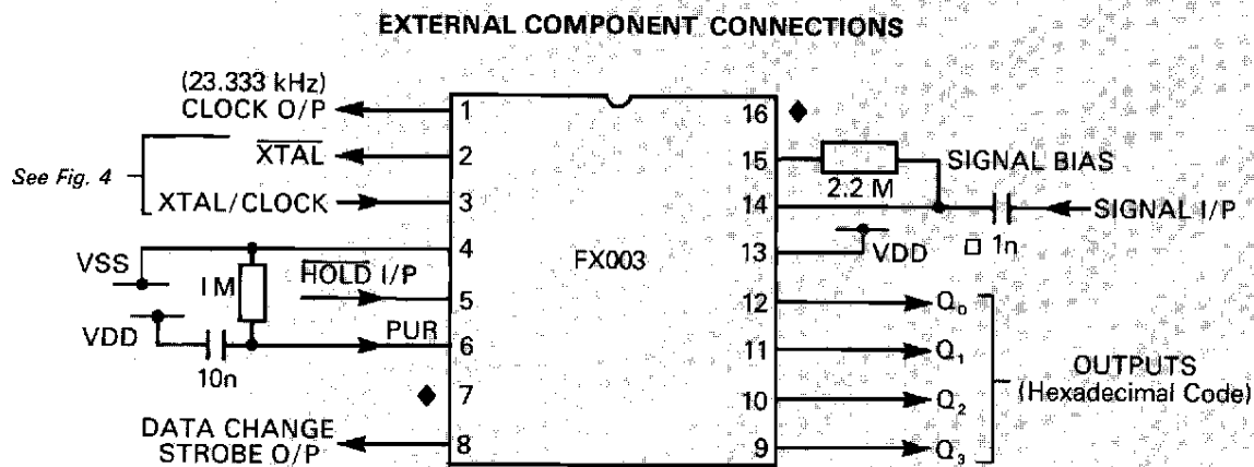
Fig. 2 Dual-In-Line
