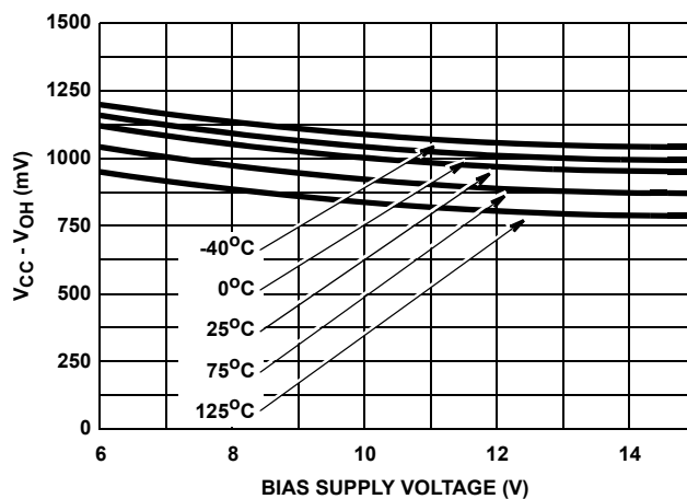
FIGURE 25. HIGH LEVEL OUTPUT VOLTAGE, V_{CC} - V_{OH} vs BIAS SUPPLY AND TEMPERATURE AT 100mA
