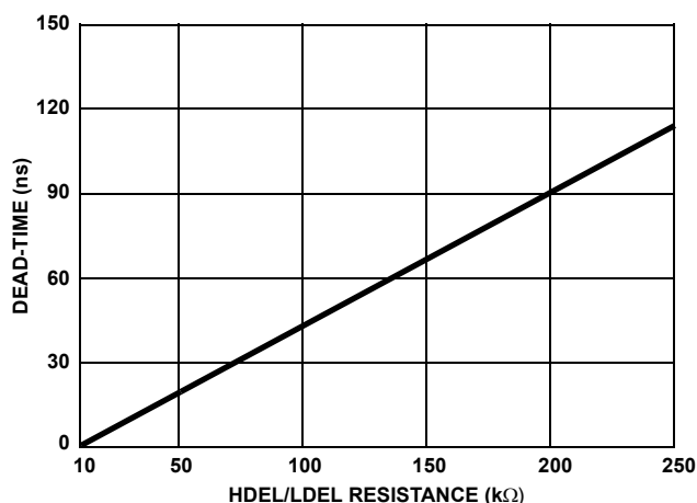
FIGURE 31. MINIMUM DEAD-TIME vs DEL RESISTANCE
