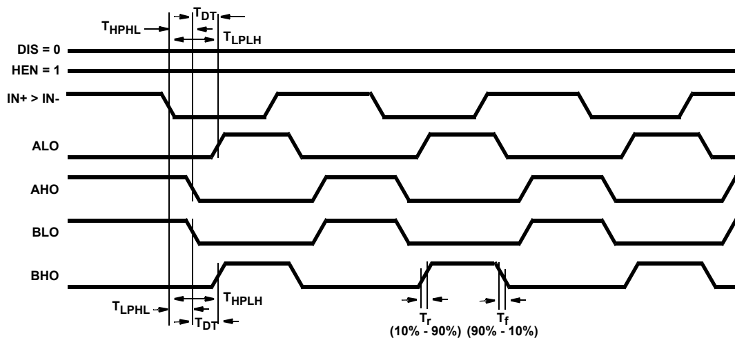
FIGURE 1. BI-STATE MODE
