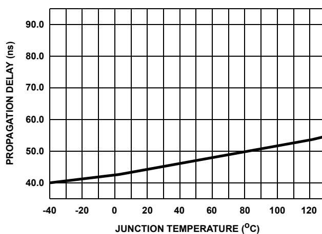
FIGURE 21. LOWER TURN-ON PROPAGATION DELAY T_{LPHL} vs TEMPERATURE
