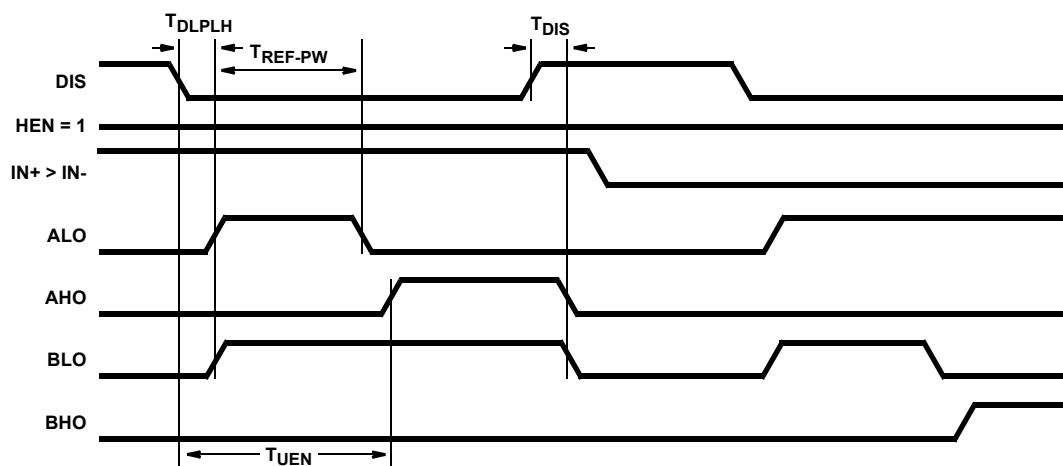
FIGURE 3. DISABLE FUNCTION
