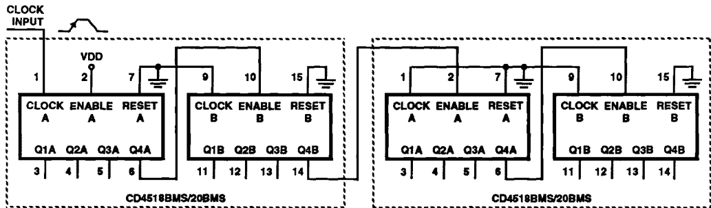
FIGURE 13. RIPPLE CASCADING OF FOUR COUNTERS WITH POSITIVE EDGE TRIGGERING
