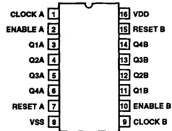
CD4518BMS, CD4520BMS TOP VIEW
