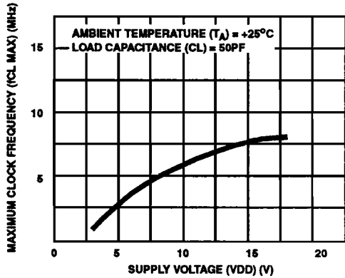
FIGURE 10. TYPICAL MAXIMUM CLOCK FREQUENCY vs SUPPLY VOLTAGE
