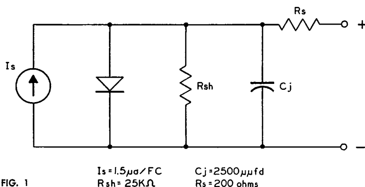
SS-300 EQUIVALENT CIRCUIT
