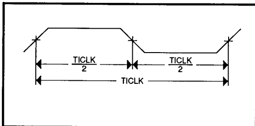
FIGURE 1: Input Clock Timing
