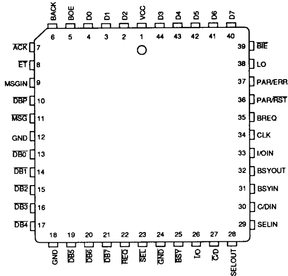
44-pin PLCC
