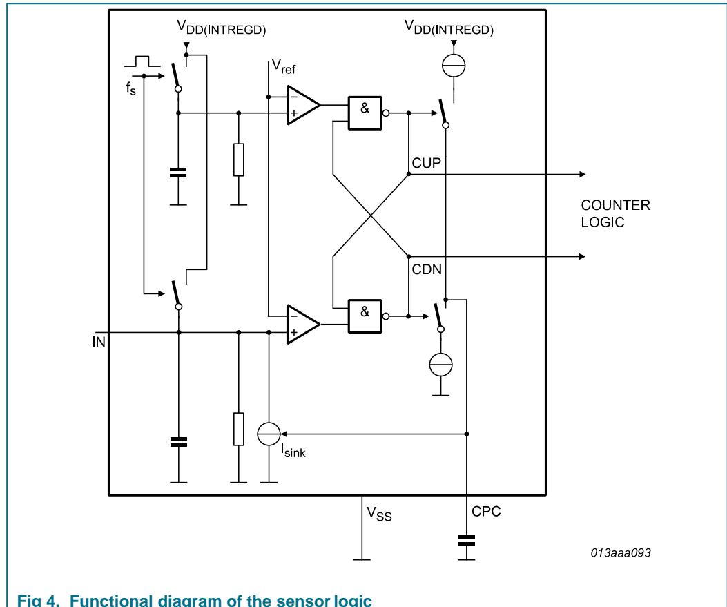
Fig 4. Functional diagram of the sensor logic
