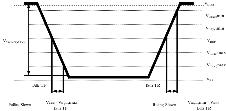
FIGURE 3 Single-ended AC Input Test Conditions Diagram
