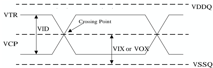
FIGURE 4 Differential DC and AC Input and Output Logic Levels Diagram
