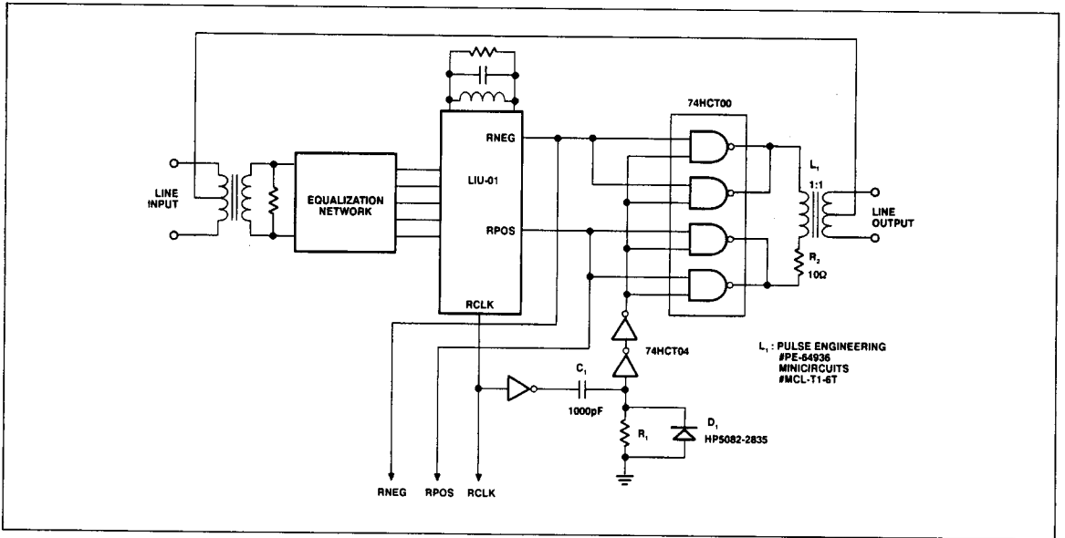
FIGURE 19: The LIU-01 acts as an in-line monitor/repeater using 74HCT00 as an output driver. D_1 , R_1 , and C_1 stretch the duty cycle of RCLK to 50%. The value of R_1 depends on the operating data rate.
