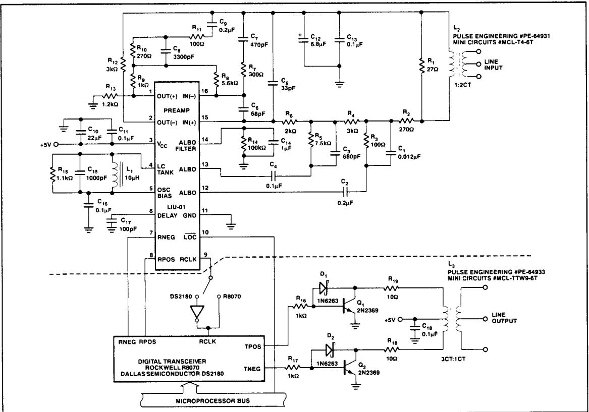
FIGURE 13: The LIU-01 enables this 4-wire transceiver to recover T1 data at 1.544Mbps/s with an input signal level varying from 0dB to less than -36dB. The ALBC/equalization network is compatible with unshielded #22AWG twisted-pair wire measuring 16p/ft.
