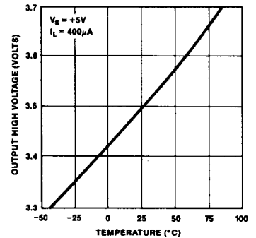
OUTPUT HIGH VOLTAGE (V OHD ) vs TEMPERATURE
