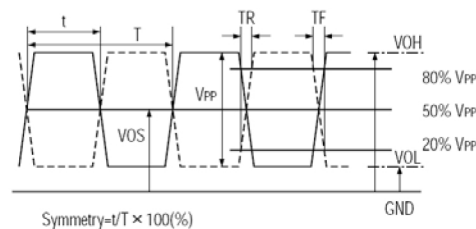
Figure 4) Output Waveform
