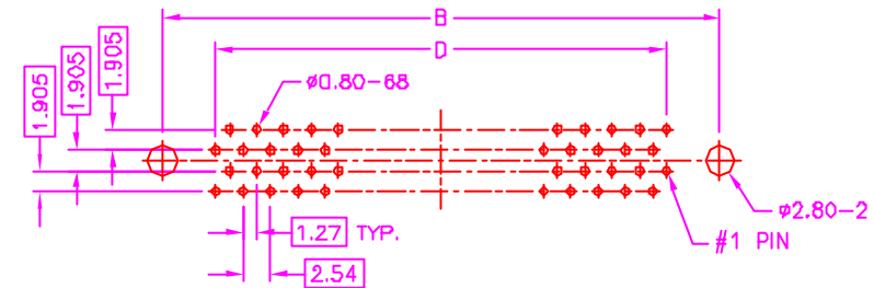
RECOMMEND P.C.B. LAYOUT (68 PINS) BOTTOM VIEW
