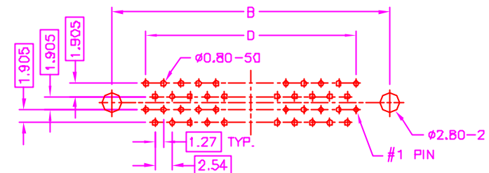
RECOMMEND P.C.B. LAYOUT (50 PINS) BOTTOM VIEW
