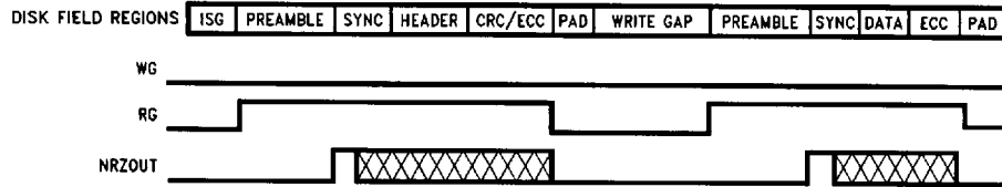
FIGURE 10. Hard Sector Read Mode Waveforms
