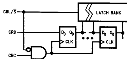
FIGURE 7. CTRL Register Block Diagram
