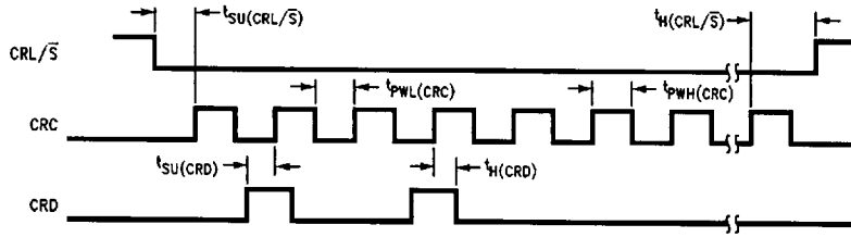
FIGURE 4. Control Register Timing Diagram
