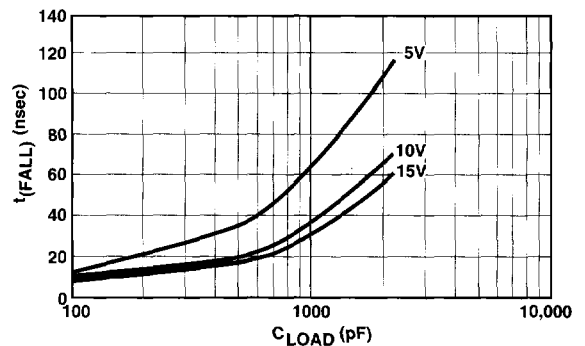
Fall Time vs. Capacitive Load
