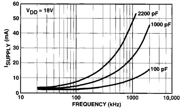
Supply Current vs. Frequency
