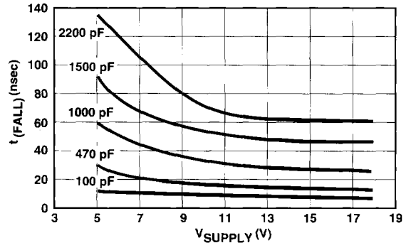
Fall Time vs. Supply Voltage
