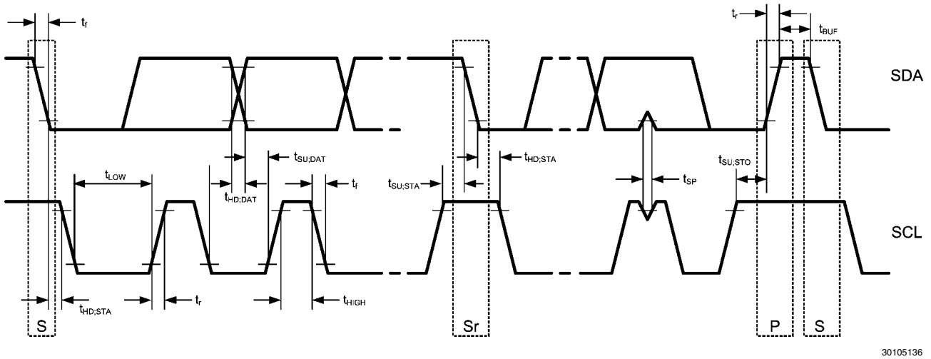
FIGURE 11. Serial Control Bus Timing Diagram
