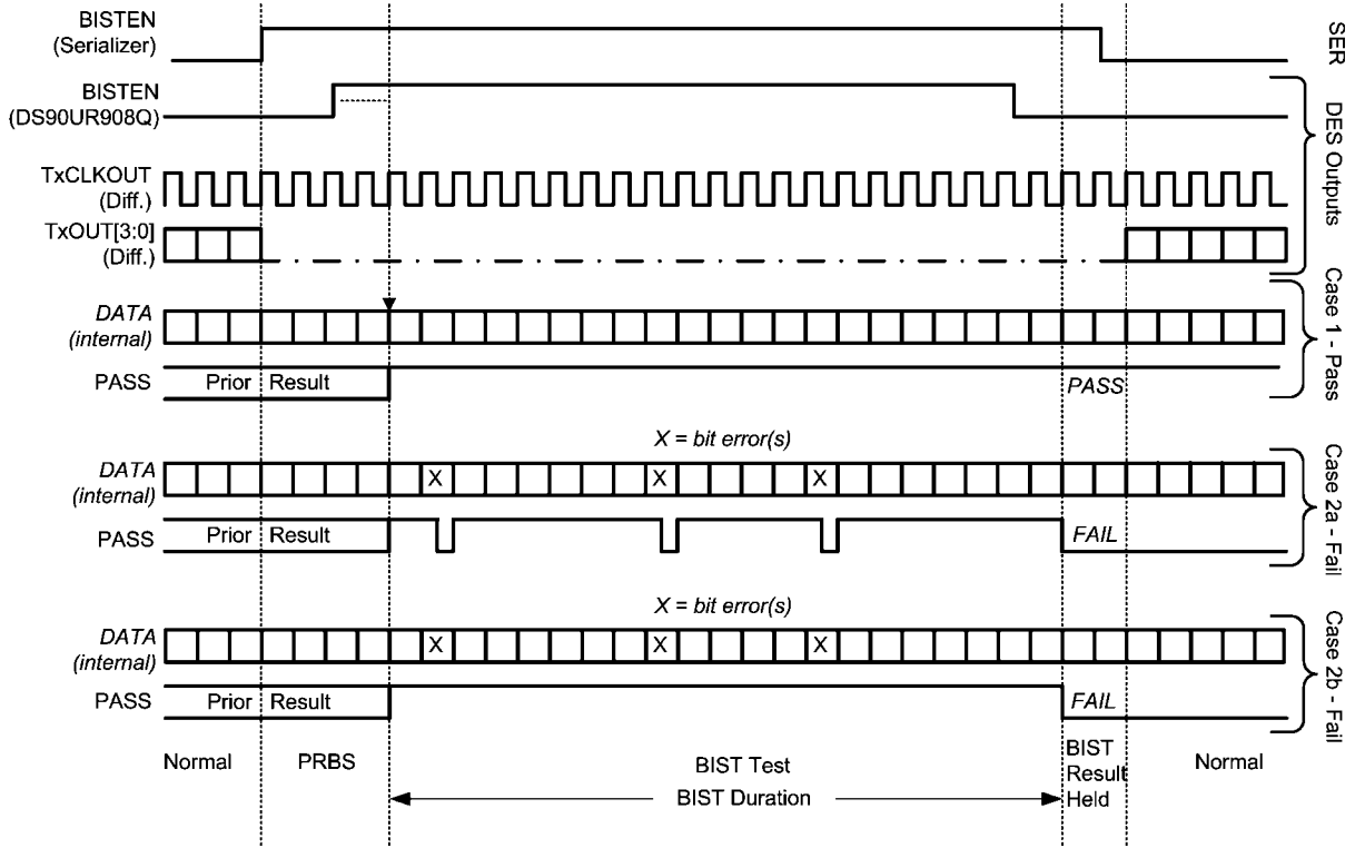
FIGURE 19. BIST Waveforms
