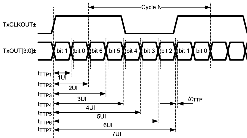
FIGURE 8. FPD-Link Transmitter Pulse Positions
