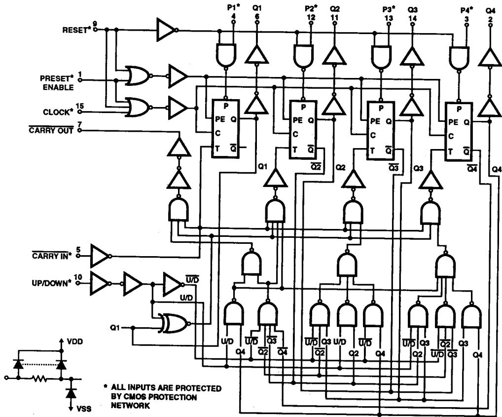
FIGURE 1. CD4510BMS
