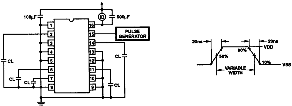
FIGURE 11. POWER DISSIPATION TEST CIRCUIT AND INPUT WAVEFORM
