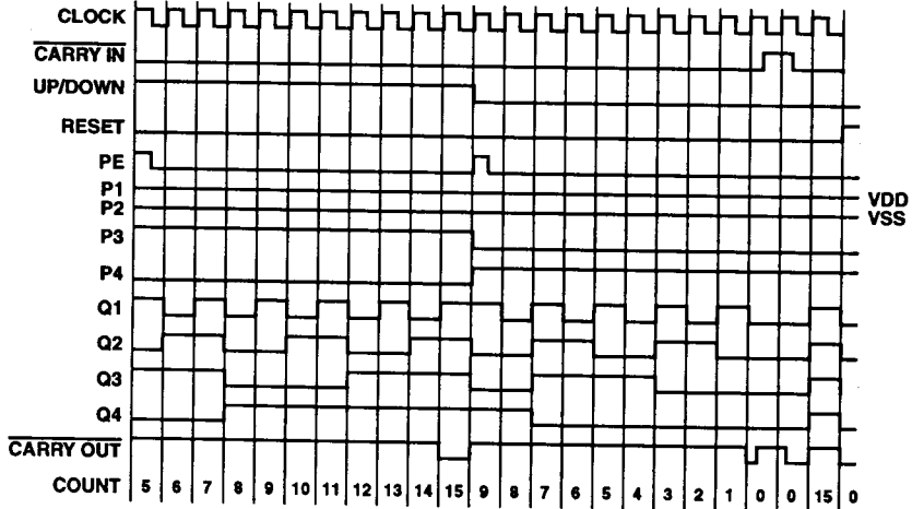
FIGURE 14. CD4516BMS
