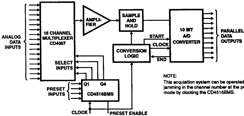
FIGURE 12. TYPICAL 16 CHANNEL, 10 BIT DATA ACQUISITION SYSTEM
