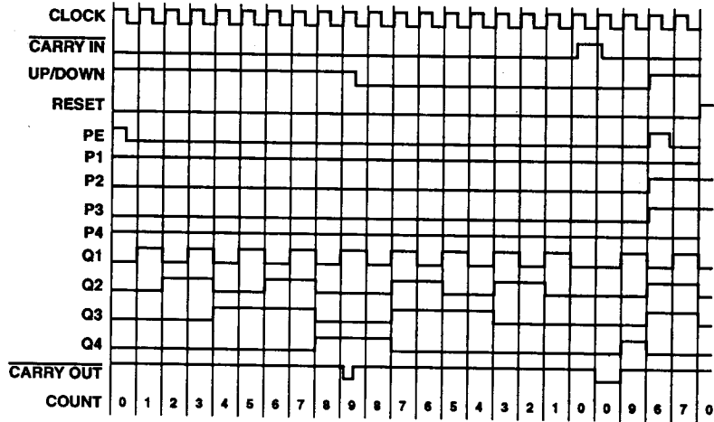
FIGURE 13. CD4510BMS
