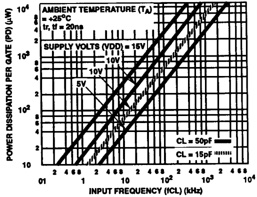
FIGURE 10. TYPICAL DYNAMIC POWER DISSIPATION vs FREQUENCY
