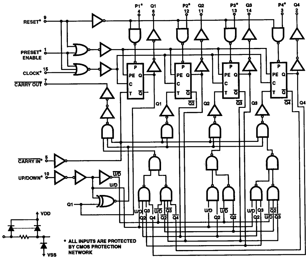
FIGURE 2. CD4516BMS
