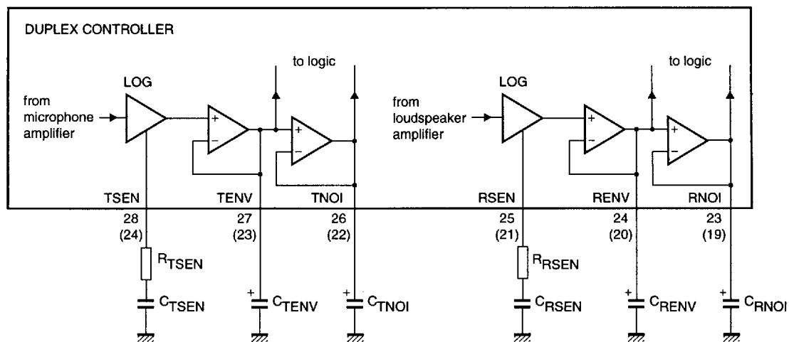
Fig.7 Signal and noise envelope detectors.
