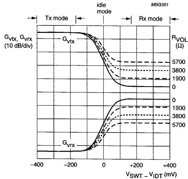
Fig.11 Switch-over behaviour.
