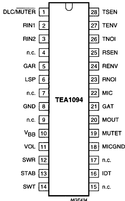
Fig.2 Pin configuration (TEA1094).
