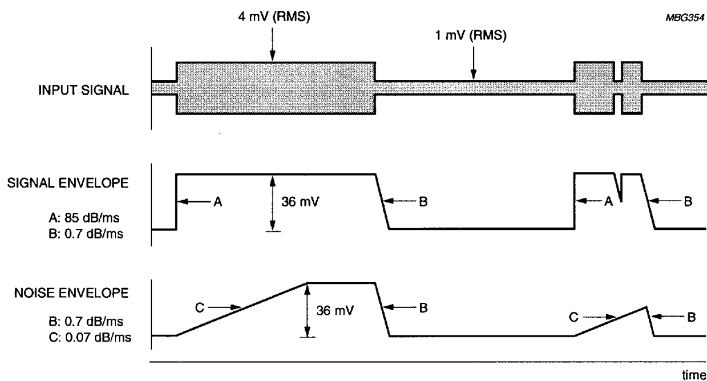
Fig.8 Signal and noise envelope waveforms.
