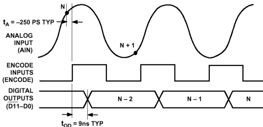
FIGURE 1. TIMING DIAGRAM
