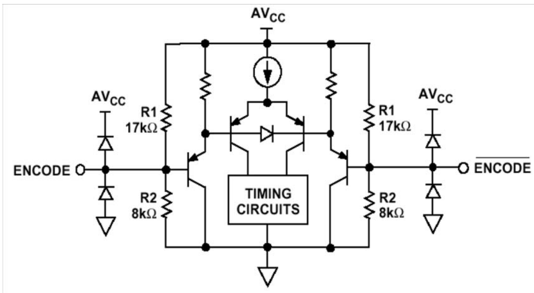
FIGURE 3. ENCODE INPUTS EQUIVALENT CIRCUIT
