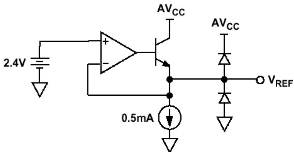
FIGURE 6. 2.4 V REFERENCE EQUIVALENT CIRCUIT
