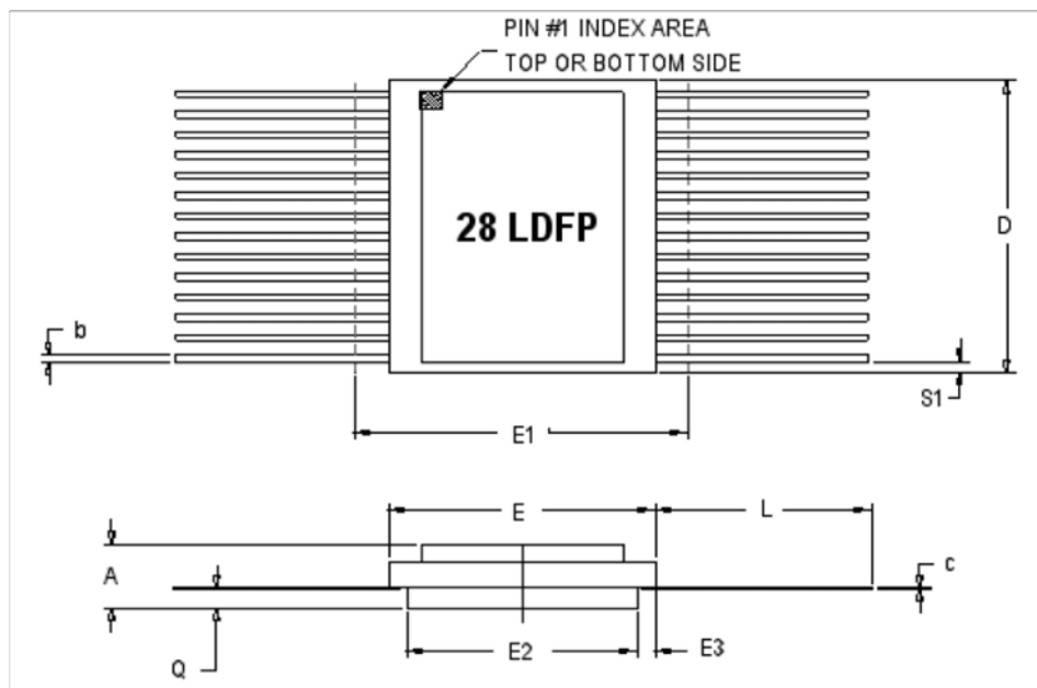
28-PIN RAD-PAK® FLAT PACKAGE
