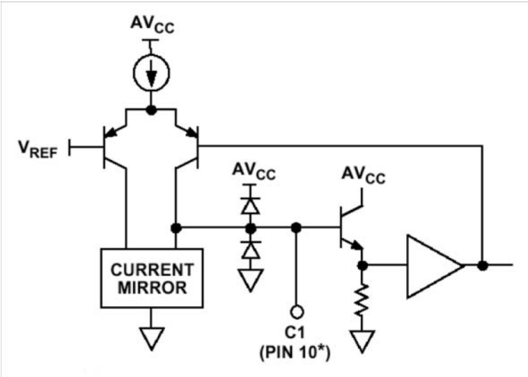
FIGURE 4. COMPENSATION PIN, C1 EQUIVALENT CIRCUIT
