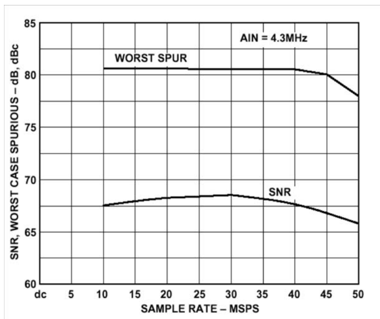
FIGURE 16. SNR WORST HARMONIC VS. ENCODE
