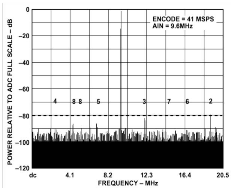
FIGURE 8. SINGLE TONE AT 9.6 MHz
