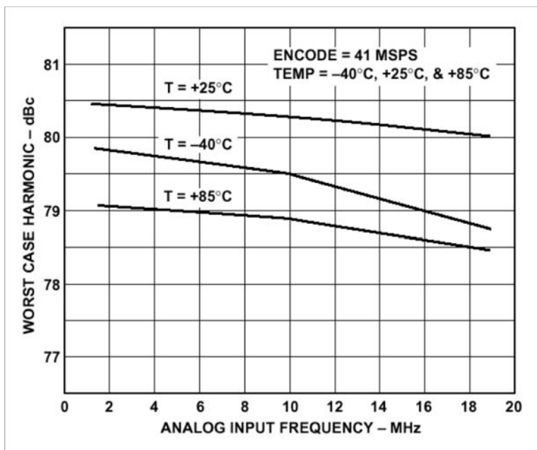
FIGURE 10. HARMONICS VS. AIN
