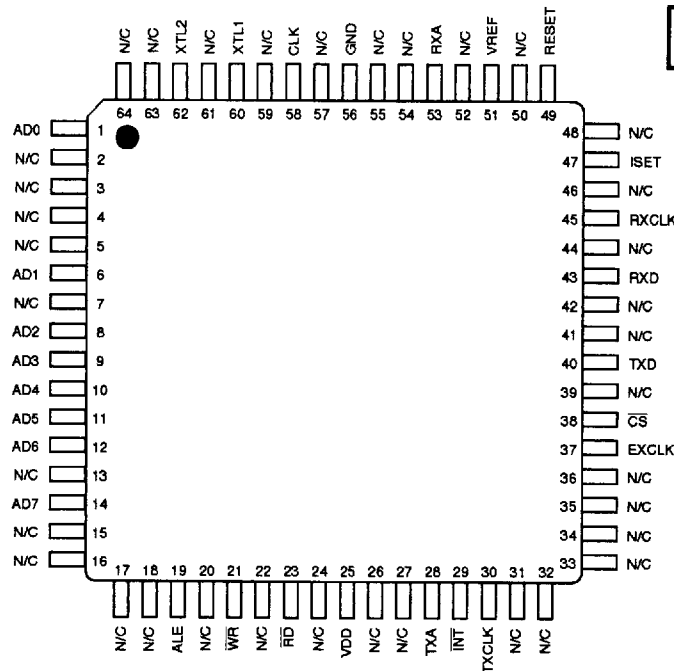
64-Lead TQFP
