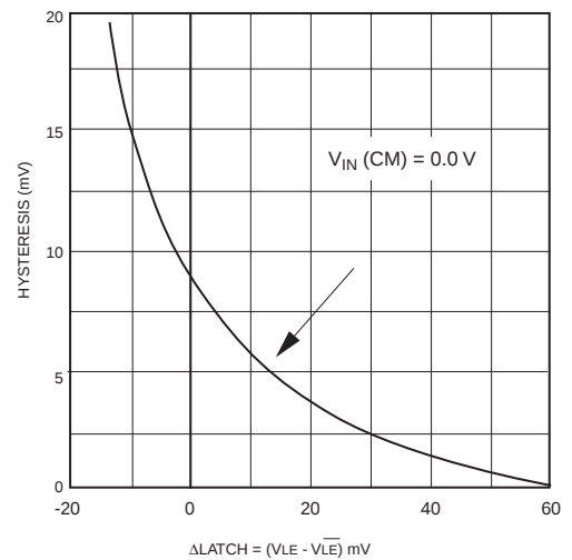
HYSTERESIS VS \Delta LATCH
