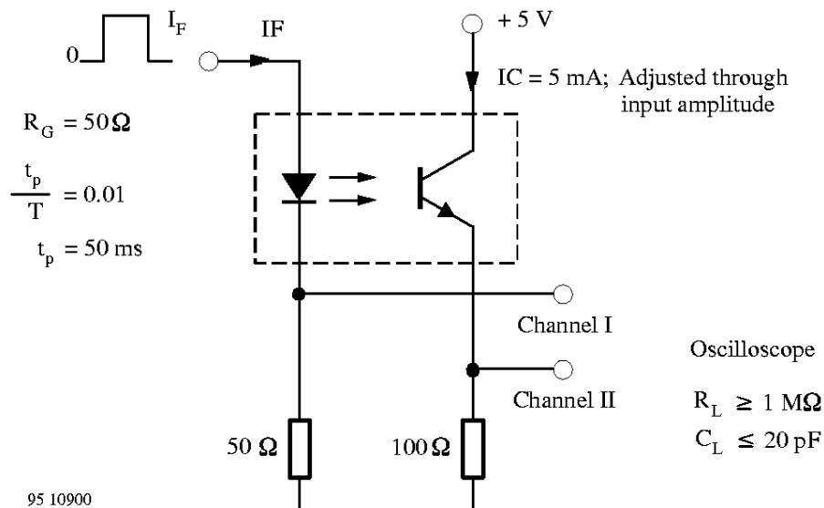
Figure 1. Test circuit
