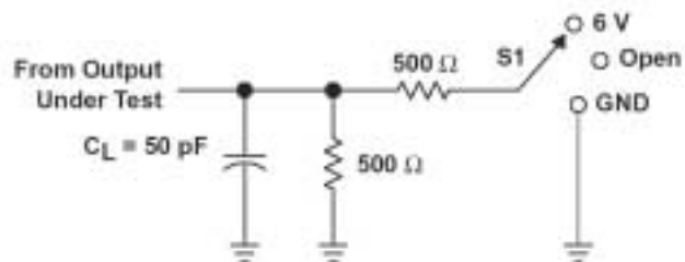
FIGURE 1. LOAD CIRCUIT
