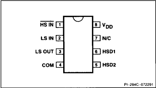
Figure 2. Pin Configuration.
