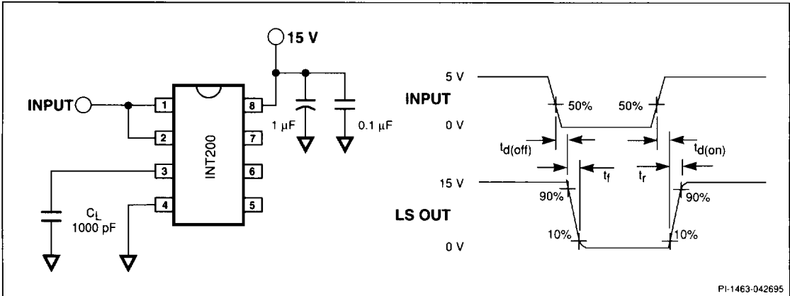
Figure 7. Switching Time Test Circuit.
