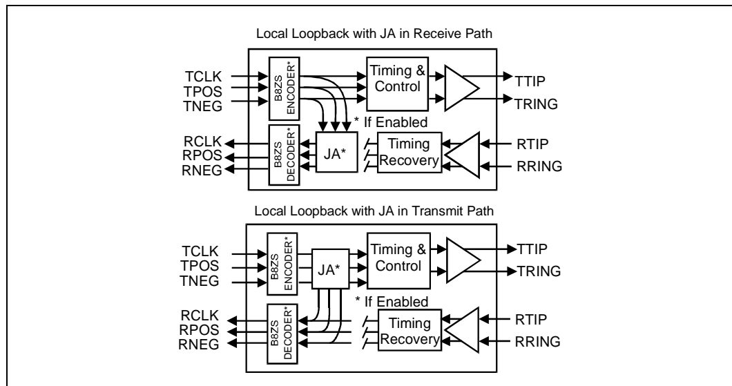
Figure 5. Local Loopback
