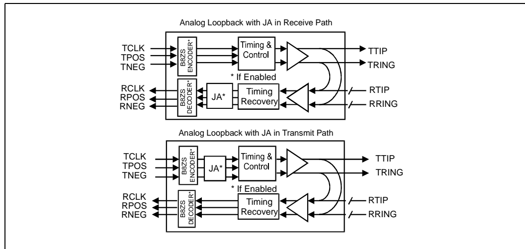
Figure 6. Analog Loopback
