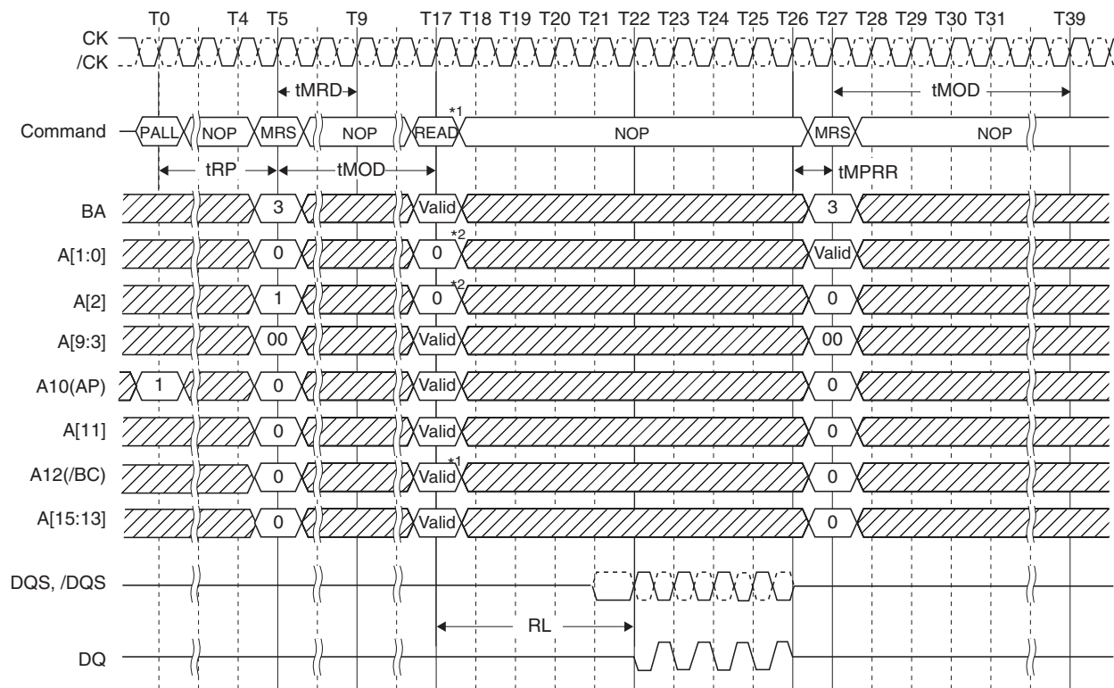
MPR Readout of Preddefined Pattern, BL8 fixed Burst Order, Single Readout
