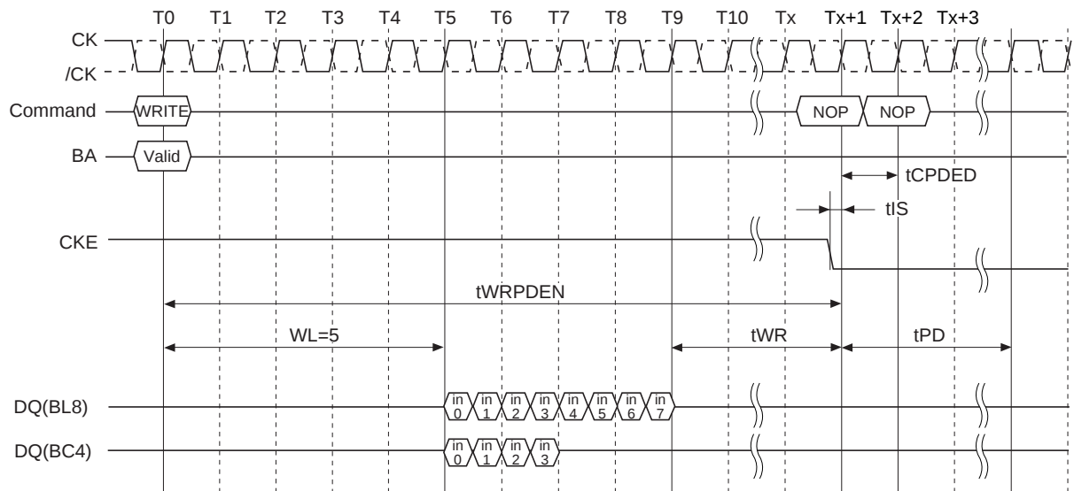
Power-Down Entry after Write
