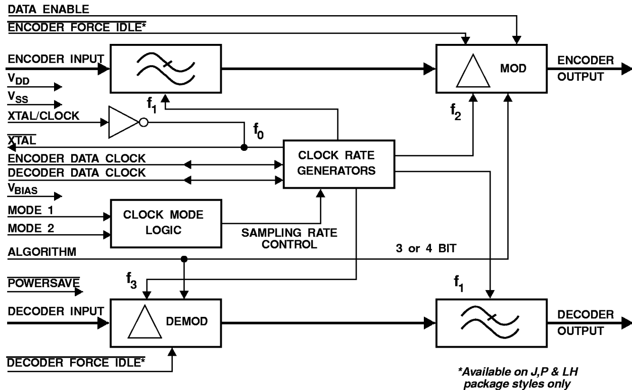
Figure 1: Block Diagram
