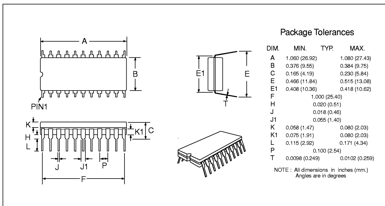
Figure 12: 22-pin Cerdip (J) Mechanical Outline: Order as part no. MX609J
