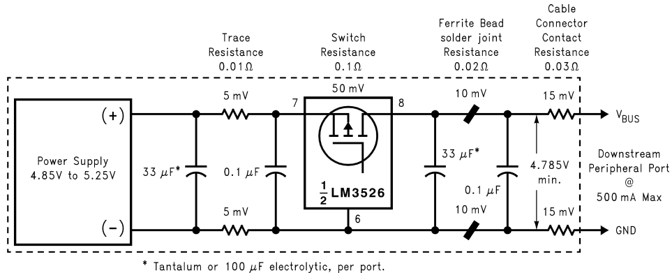
FIGURE 2. Self-Powered Hub Per-Port Voltage Drop
