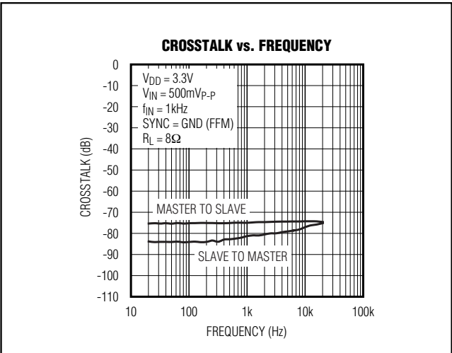
Figure 8. Master-Slave Crosstalk
