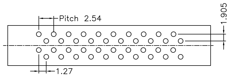
PCB HOLE
