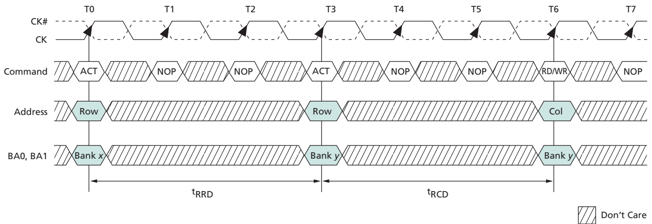
Figure 26: Example: Meeting t^{RRD} ( t^{RCD} ) MIN When 2 < t^{RCD} ( t^{RRD} ) MIN/ t^{CK} \leq 3
