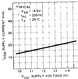
I_{DD4} (PAGE-MODE) vs V_{DD} SUPPLY VOLTAGE
