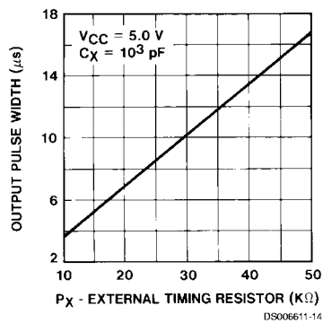
FIGURE 3. Pulse Width vs Timing Resistor
