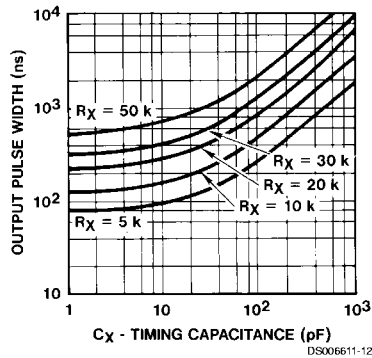
FIGURE 1. Output Pulse Width vs Timing Resistance and Capacitance for C_X < 10^3 \text{ pF}
