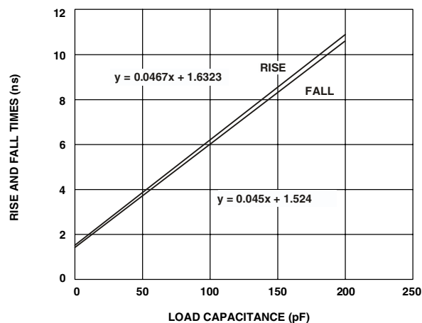
Figure 31. Typical Output Rise/Fall Time (20%-80%, V_{DDEXT} = \text{Max} )
