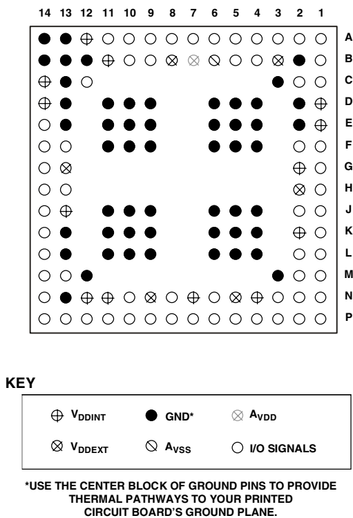
Figure 34. 136-Ball Mini-BGA Pin Assignments (Bottom View, Summary)
