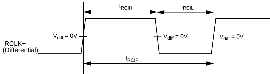
Fig1. Differential CLKIN
