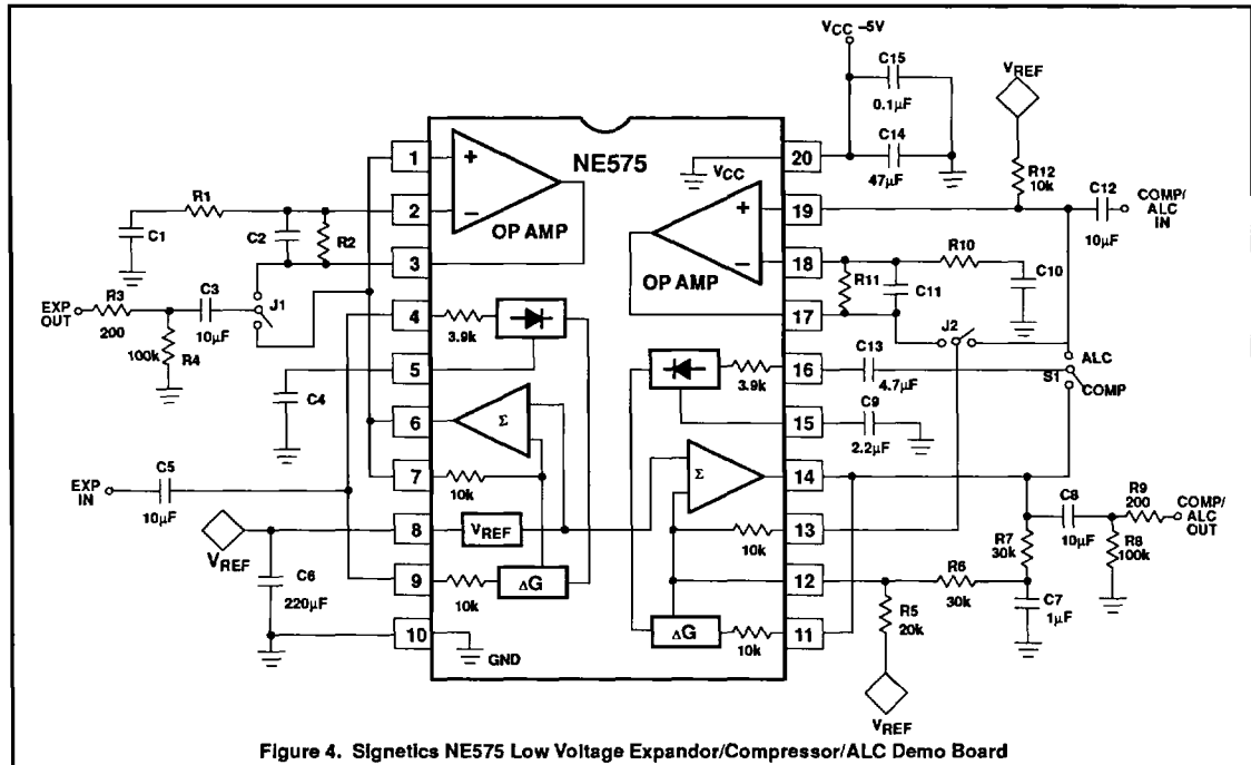
Figure 4. Signetics NE575 Low Voltage Expandor/Compressor/ALC Demo Board
