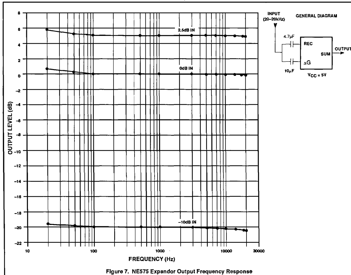
Figure 7. NE575 Expander Output Frequency Response
